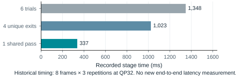
Figure S27. The decision path has an encoder cost. a , Stages required for source-error-based selection, with prefix reuse across candidate exits. b , Historical table-construction upper medians over 24 pooled trials, without invented uncertainty bars. c , A fixed held-out control and per-frame source calibration require different information. This is a stage analysis, not an end-to-end speedup.
