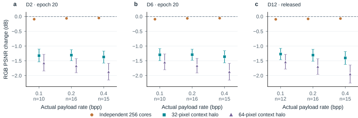
Figure S31. Charge repeated context to the transmitted rate. RGB PSNR changes from the same full-frame model at matched actual payload rate. Each depth uses the common supported images across full frame and all three patch variants; counts are shown and the vertical scale is shared. Intervals resample paired images. D2/D6 are interim epoch 20 models; D12 has different released training provenance. The experiment holds depth fixed within every contrast and makes no adaptive-routing or runtime claim.
