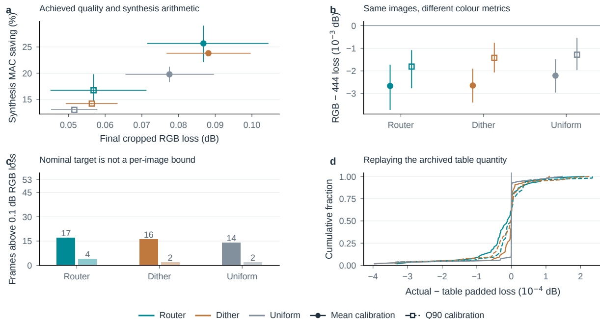
Figure S28. Carry the fixed decision through to the actual image. All 53 sequences at QP32, with no outcome-based exclusions. a , Achieved RGB loss and synthesis MAC saving with conditional 95% sequence-bootstrap intervals; these points are not an equal-quality frontier. b , RGB-minus-444 loss on the same support and reference. c , Counts above the nominal numerical threshold; pale bars denote Q90 calibration. d , Actual-minus-table loss on padded support. Mean and Q90 controls use a different calibration reference and metric from the cropped RGB report. The paired router-dither saving intervals include zero under both controls.
