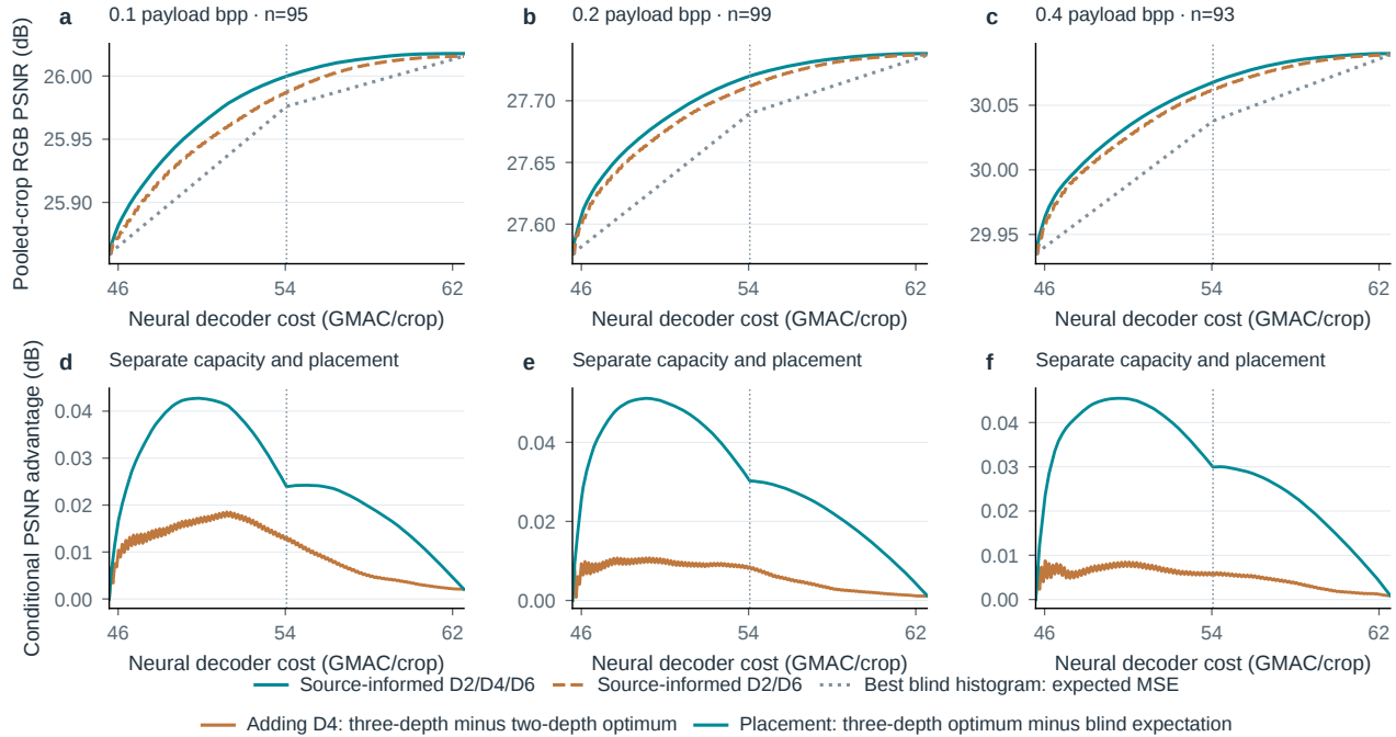
Figure S24. Separate the value of capacity choices from their assignment. Top: exact whole-crop allocation under a shared neural-decoder MAC budget. Bottom: incremental D4 option value and assignment premium over the best source-calibrated blind histogram’s expected MSE. Vertical guides mark the uniform-D4 budget. The curves use interpolated equal-rate quality and contain neither patch entropy resets nor a trained MLP. They are not within-image routing results or runtime frontiers.
