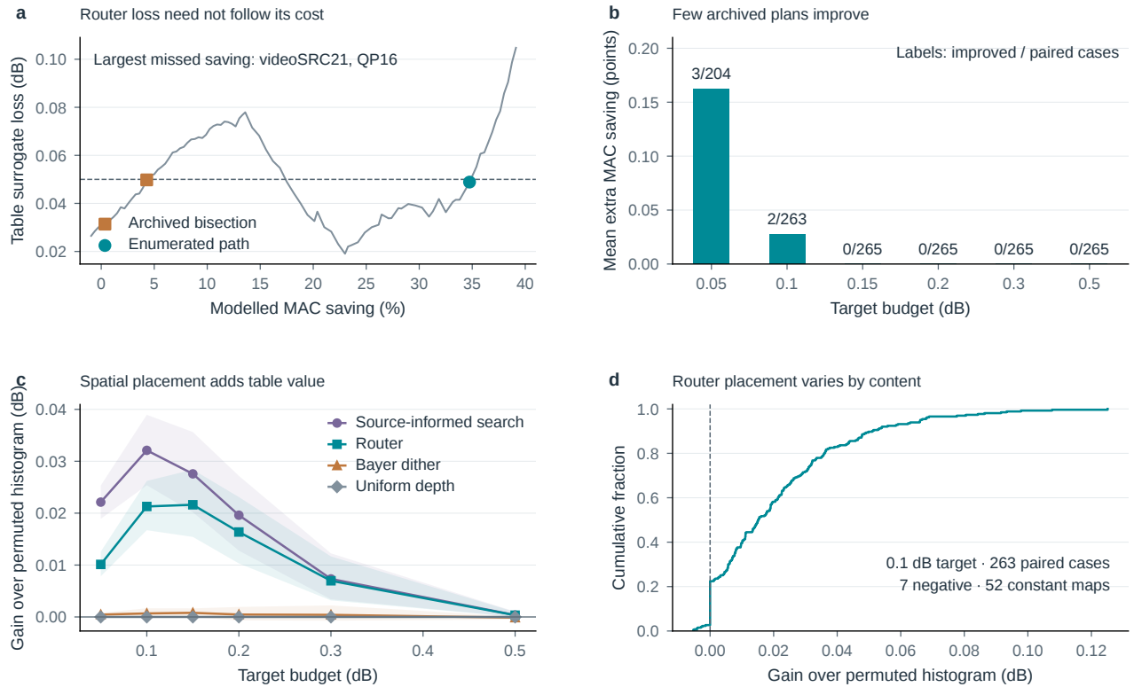
Figure S15. Control-path and assignment diagnostics. a , The explicitly selected largest missed router saving illustrates non-monotone table loss. b , Mean paired improvement from enumerating the router path; labels show improved and paired counts. Newly feasible cases are excluded from these means. c , Exact expected-shuffle comparison at unchanged exit histograms, with 95% sequence-cluster intervals. d , Router placement-gain distribution at 0.1 dB. All results are CPU analyses of padded error tables; none measures new final-image quality or latency.
