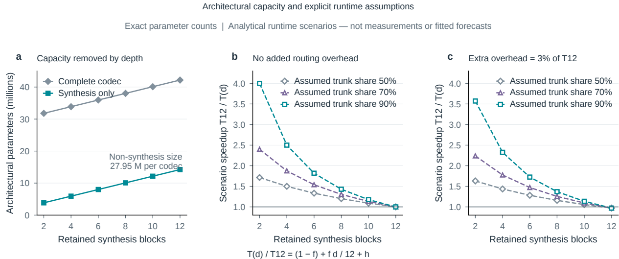
Figure S26. A transparent design-space illustration for unfinished experiments. a , Exact architectural parameter counts. b,c , Analytical runtime sensitivity to assumed trunk-time share and added overhead. Open markers and dashed lines denote assumptions, not measurements or fitted forecasts. No quality or bitrate outcome is assigned to an unfinished model.
