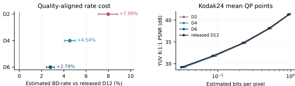
Figure S18. The completed independent codecs approach the release as depth grows. Left, per-image YUV 6:1:1 BD-rate cost on the four-model common PSNR interval; bars are 95% paired-image bootstrap intervals ( n = 24 ). Right, mean five-QP operating points on Kodak24. Rates are deterministic entropy estimates, not actual bitstreams. Released D12 differs in training history from the three scratch models.
