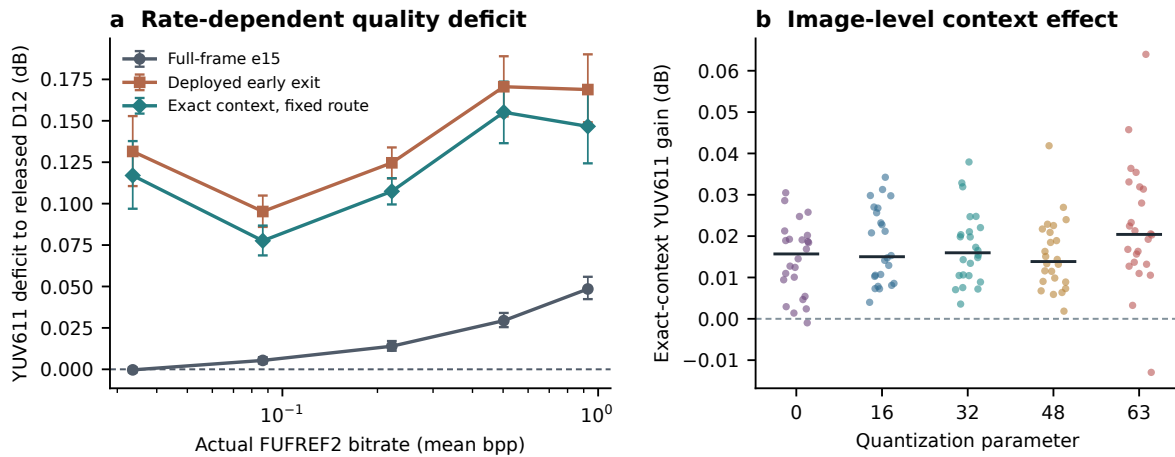
Figure S13. Kodak24 exact-context transfer at unchanged real bitrates. a , Mean YUV611 deficit to released D12 versus actual FUFREF2 bitrate for full-frame e15, diagnostic exact-context routing, and the deployed path. Vertical separations add to the released-to-deployed gap. Error bars are paired 24-image bootstrap 95% intervals; the released decoder is at zero deficit by definition. b , Per-image YUV611 gain from replacing zero-halo-plus-repair with clipped exact context and no repair, at each QP; dark bars mark medians. The exit maps remain fixed. No BD-rate or latency claim follows from this reconstruction-only counterfactual.
