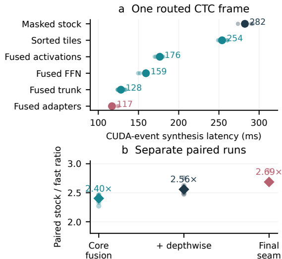
Figure S37. An implementation gain on one real routed frame. a , Six shuffled, paired CUDA-event trials of consecutive kernel stages. Dots are trials and large marks are medians. b , Three separately timed implementations; ratios are paired within each run but cannot be compared as an incremental ablation across runs because GPU contention changed. CTC videoSRC05 at QP32, 1920 \times 1080 valid pixels padded to 2048 \times 1280 , with exit-6/8/10/12 tile counts 13/20/4/3. The GPU was shared with training.
