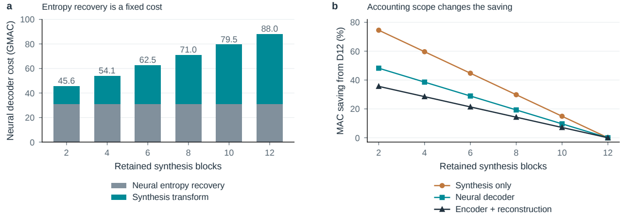
Figure S19. The arithmetic denominator changes the apparent saving. a , Synthesis varies with depth while neural entropy recovery stays fixed. b , The same architectural intervention under three accounting scopes. Counts use 512 \times 512 input and one MAC per multiply-accumulate; they are not observed kernel times. D8/D10 are architecture-only controls. Encoder totals include reconstruction but omit rANS, elementwise work, transfers and control overhead.
