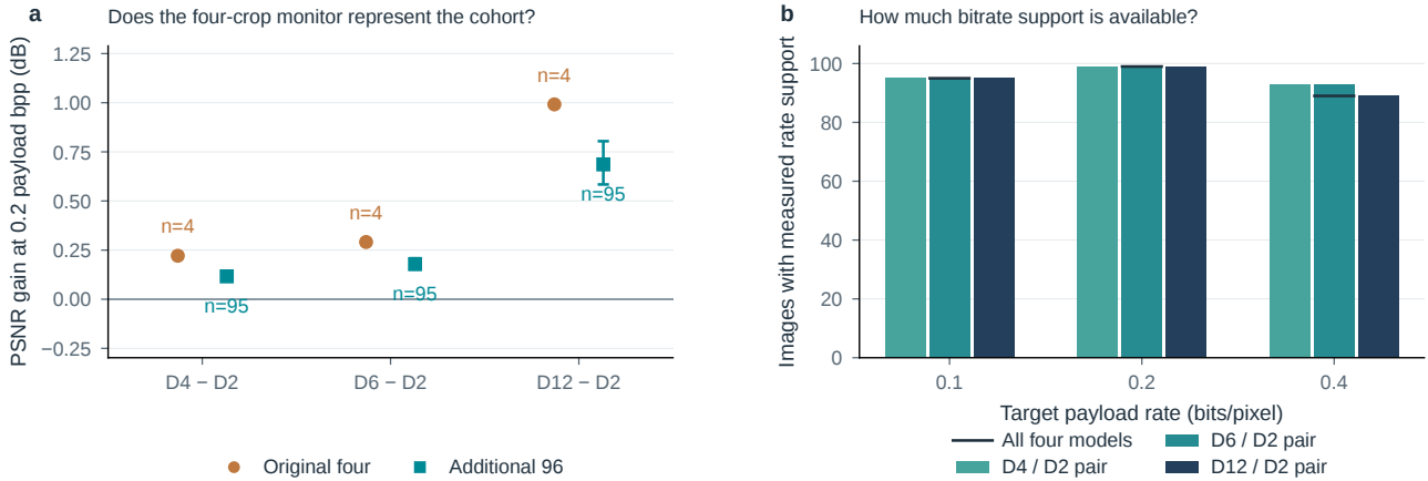
Figure S21. Coverage is part of the result. a , Original monitor crops and additional images at 0.2 payload bpp, restricted to four-model common support. We do not estimate uncertainty from the four-crop subset. b , Pairwise and four-model supported counts at each target rate. A changing cohort is made explicit rather than filled by extrapolation.
