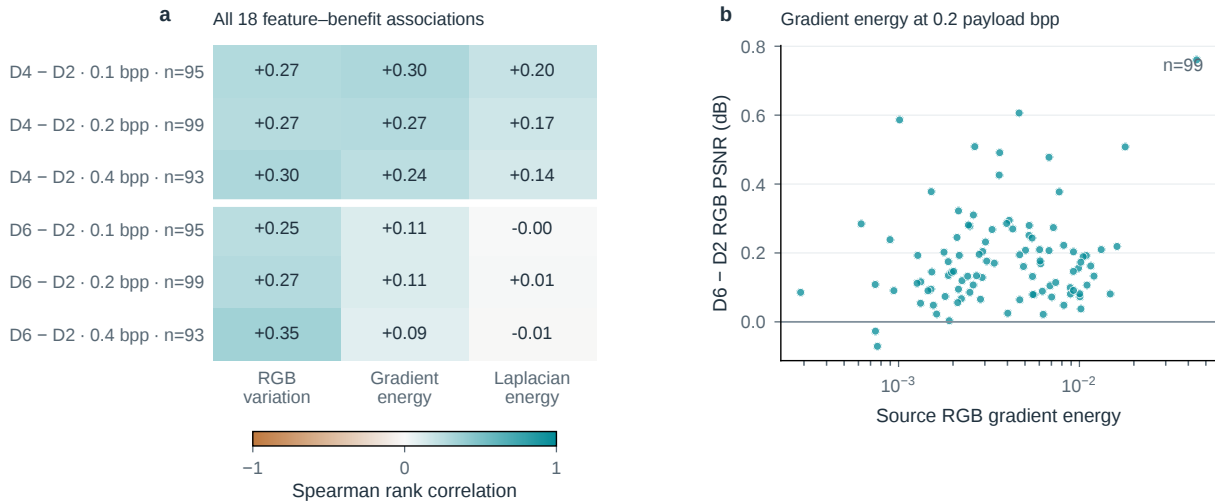
Figure S25. Cheap complexity measures do not directly identify the useful expert. All 18 specified feature/depth/rate combinations are shown, with supported image counts. The scatter panel was fixed to gradient energy versus D6–D2 at 0.2 bpp before inspecting the associations. These are correlations with interim equal-rate benefits, not router accuracy or causal feature effects.
