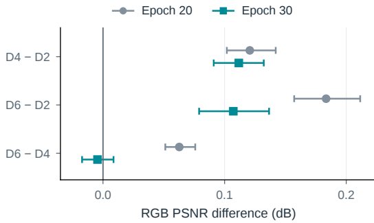
Figure S23. Intermediate depth ordering changes during training. Paired RGB PSNR differences at 0.2 actual payload bpp on the same 99 images. Epochs 20 and 30 are retained without quality-based selection. Intervals are 95% image-bootstrap intervals at fixed weights, excluding training-seed uncertainty. No rate extrapolation.
