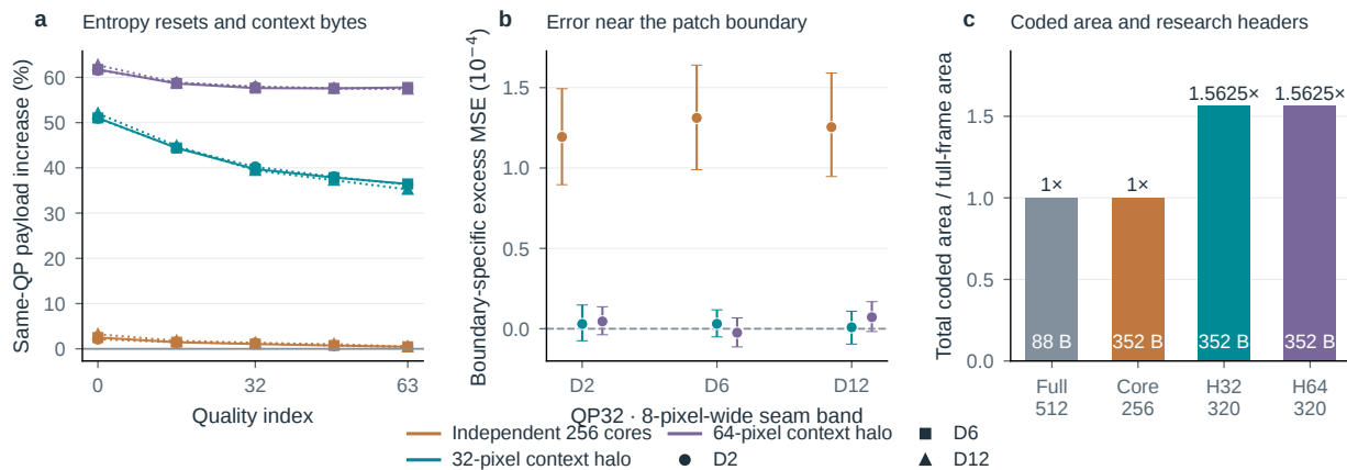
Figure S32. A better seam and a better codec are different outcomes. a , Same-QP payload increase over the full-frame model. b , At QP32, patch-minus-full MSE in the central 8-pixel seam band, minus the corresponding interior excess. c , Exact coded area and research-header bytes. Halo32 and halo64 have equal coded area under this padding policy, but different real context. Area ratios are not latency ratios, and same-QP seam diagnostics are not equal-rate quality comparisons.
