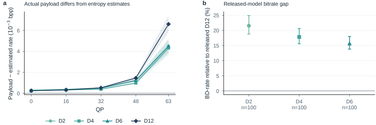
Figure S22. Estimated entropy and emitted bytes are separate quantities. a , Actual rANS payload minus entropy estimate, excluding the research header. b , Mean per-image BD-rate against the released anchor on each image's four-model common PSNR interval. Intervals resample images; no uncertainty from independent training seeds is represented.
