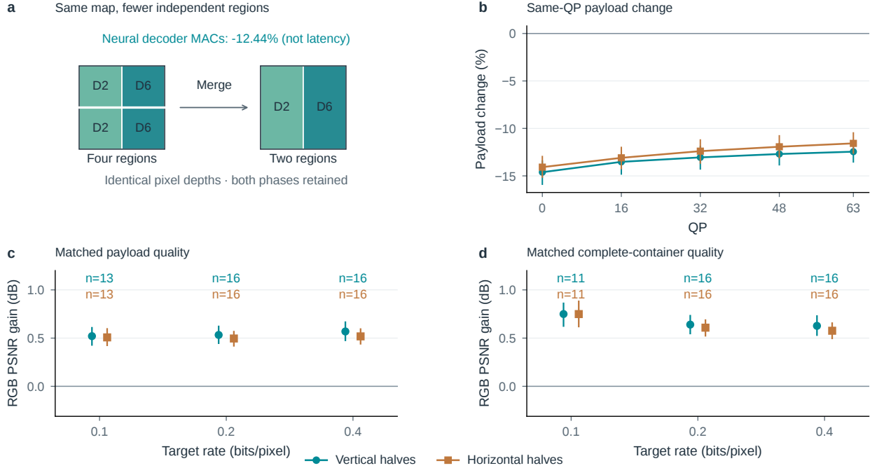
Figure S35. Better region execution without a better selector. a , One phase of the fixed depth-map control; every pixel keeps its D2 or D6 assignment. b , Same-QP relative payload change after coalescing. c,d , RGB PSNR gain at matched payload and complete-container rate, on shared vertical scales. Complementary phases are averaged within image before 95% paired-image bootstrap intervals. Counts show the common support of both phases and implementations, without extrapolation. The 800 outputs include unmerged checkerboards; those have no adjacent same-depth regions to combine. CPU FP32 research streams and epoch-20 weights are used throughout; this is neither learned routing nor a runtime benchmark.
