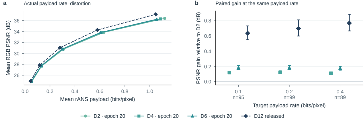
Figure S20. Shallow models are close, but not identical, at equal coded rate. a , Mean RGB PSNR and actual payload over all 100 crops at five QPs; joining lines are visual guides. b , Per-image interpolation and paired differences on four-model common support, with 95% image-bootstrap intervals. D2/D4/D6 are frozen epoch-20 models; released D12 is not matched in training history. These measured streams establish an interim CPU rate–distortion comparison, not final quality or native runtime.
