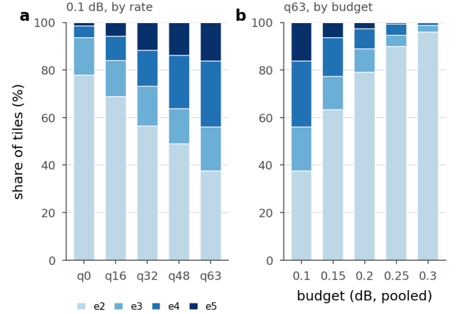
Figure 46. How the ladder fills up. a , exit shares at the 0.1 dB budget as the rate rises. b , exit shares at q63 as the budget loosens, until at 0.3 dB 96% of tiles are already at the shallowest exit and there is almost nothing left to allocate. Both panels are pooled over the test set.
