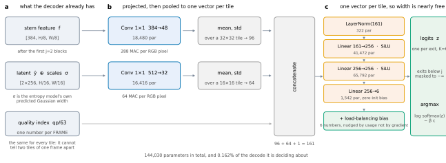
Figure 57. The router head. a , the three things it reads, all already held by the decoder at the moment the decision is needed. b , each projected by a 1×1, then reduced to one vector per tile by its mean and standard deviation. c , a three-layer perceptron, one pass per tile. Every shape and parameter count in the figure is read off the module when the figure is drawn.
