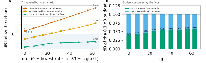
Figure 52. The tiling penalty across the whole rate range, every tile at full depth, so this is the floor and nothing else. a, the steps that reduce it, of which the two that matter cost no arithmetic; the largest single factor is training the ladder with the seam present. b, the floor as a share of the 0.1 dB budget: it is charged inside the budget and consumes a growing part of it as the rate rises, which is one of the two reasons the saving falls with rate.
