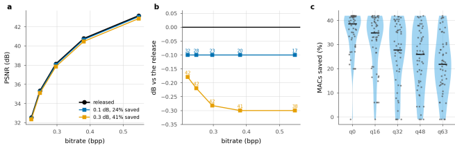
Figure 8. The plane a codec is read on, and the spread behind the mean. a, operating points against the released curve. b, the same with the quality axis expanded; labels are compute saved. c, per sequence at a matched point near 0.1 dB; one dot per sequence, bar is the median.
