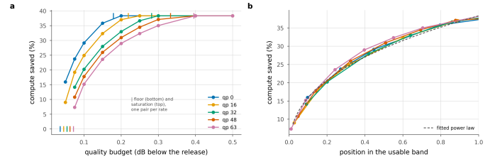
Figure 24. The band is the rate dependence. a, saving against the budget, with each rate's floor and saturation point ticked. b, the same with the budget axis rescaled onto each rate's own band. Five curves become one; dashed is the one-parameter power law fitted to all of them.
