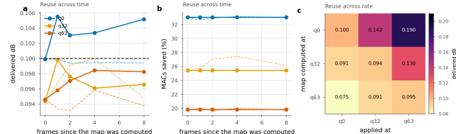
Figure 15. Reusing an exit map. Solid is the transferred map, dashed the one recomputed in place. a, b: reuse across frames of the same sequence. c: reuse across quality index; the entry is the delivered distortion against a 0.1 dB budget.
