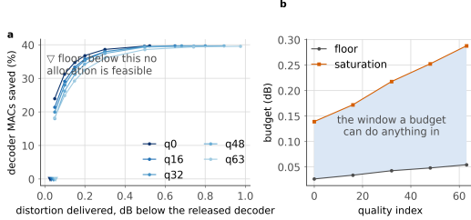
Figure 26. The window a budget works in. a , saving against the distortion actually delivered, per rate. Every curve begins at a floor, below which no allocation meets the budget, and flattens at a saturation point, above which a looser budget buys nothing. b , those two limits against rate. The shaded band is the only region in which a budget is a design choice rather than a formality.
