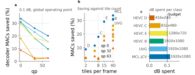
Figure 21. Saving by test class at one global operating point. \lambda is bisected once so the whole set lands on the budget, exactly as it would be in deployment; each class is then reported at that \lambda . The ordering follows tile count, not content.
