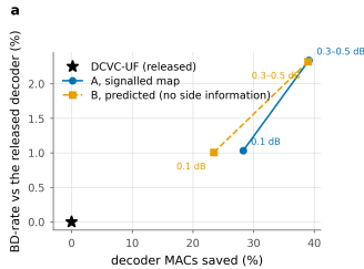
Figure 37. What the saving costs in rate. BD-rate against the released decoder, against the decoder MACs saved, for both configurations at the three budgets; each point is labelled with the budget that produced it. The star is the released decoder itself: no saving, no cost. Anchored on the same bitstream, so a BD-rate here is the price of decoding one file with fewer operations, not one codec against another.
