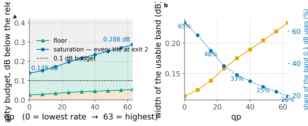
Figure 22. Three regions, and only the middle one is a design choice. Below the floor no allocation meets the budget; above saturation every tile already takes the cheapest exit. The 0.1 dB budget uses 65% of the band at the lowest rate and 20% at the highest.
