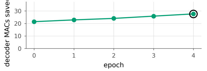
Figure 38. The run had not converged. Measured saving at the 0.1 dB budget on the 53 test frames, hook-counted, one point per completed epoch of the reported run. The circled point is the checkpoint this paper reports. The training loss over the same epochs is flat; the supplement shows the two together.
