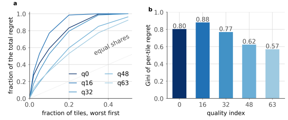
Figure 31. The loss is concentrated. a , the share of the total regret carried by the worst fraction of tiles, per rate; the dotted line is what an even spread would look like. b , the same as a Gini coefficient. At every rate a small minority of tiles carries most of what staying silent costs, which is why signalling a fraction of the map recovers most of the gap.
