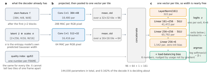
Figure 10. The router head. a , the three things it reads, all already held by the decoder. b , each projected by a 1 \times 1 , then reduced to one vector per tile by its mean and standard deviation. c , a three-layer perceptron, one pass per tile. Every shape and parameter count is read off the module when the figure is drawn.
