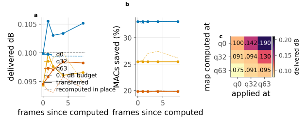
Figure 34. Reusing an exit map. Solid is the transferred map, dashed the one recomputed in place. a , b : reuse across frames of the same sequence. c : reuse across quality index; the entry is the delivered distortion against a 0.1 dB budget.
