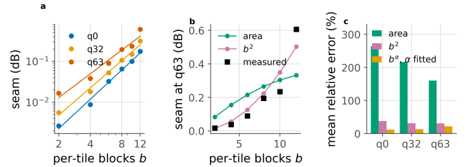
Figure 12. The seam against per-tile depth. a , the measurement with the fitted power law. b , both models against q63, one free scale each. c , mean relative error. The area fraction saturates once the border reaches every pixel; the penalty does not.
