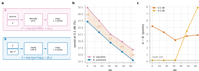
Figure 16. Who decides. (a) A holds the source, so it can decode all K exits per tile and pick the true minimiser; it signals the map at ~90 bits/frame. B never sees the source — a 144 K-parameter head reads \hat{y} , the entropy scales and qp — and signals nothing. (b) Saving at 0.1 dB; shading is what a bit-exact bitstream costs. (c)
