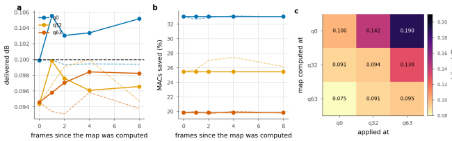
Figure 19. Reusing an exit map. Solid is the transferred map, dashed the one recomputed in place. a, b: reuse across frames of the same sequence. c: reuse across quality index; the entry is the delivered distortion against a 0.1 dB budget.
