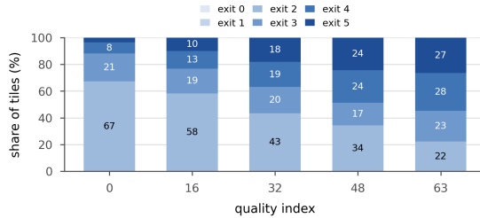
Figure 6. Where the tiles actually go, at the 0.1 dB budget, pooled over the whole test set. At the lowest rate two thirds of tiles take the cheapest available exit; at the highest only a fifth do and a quarter need the deepest. The allocation is not degenerate at either end, which is what makes the choice worth making.
