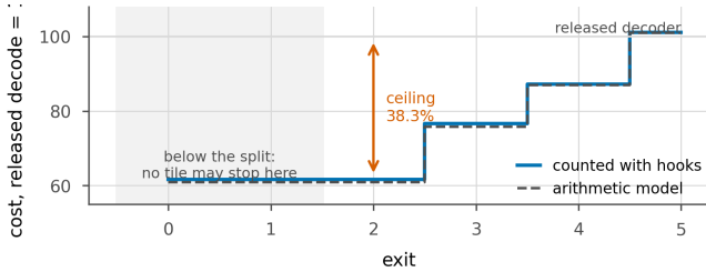
Figure 5. The ladder, priced. What a tile costs at each exit, as a percentage of one released decode, counted with hooks on the executed pass and beside the arithmetic model the argmin uses. Exits below the split depth are not distinct, because the first j groups run for every tile whatever it does. The deepest exit costs slightly more than the release, which is the full-frame deblocking pass. Reported savings in this paper are the hook count.
