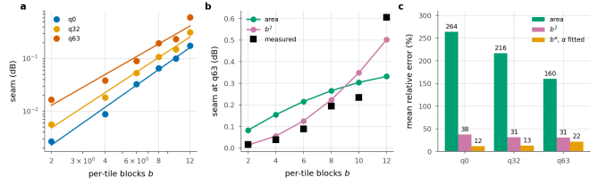
Figure 11. The seam against per-tile depth. a , the measurement with the fitted power law. b , both models against q_{63} , one free scale each. c , mean relative error. The area fraction saturates once the border reaches every pixel; the penalty does not.
