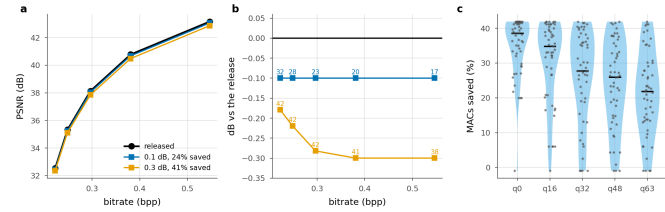
Figure 15. The plane a codec is read on, and the spread behind the mean. a , operating points against the released curve. b , the same with the quality axis expanded; labels are compute saved. c , per sequence at a matched point near 0.1 dB; one dot per sequence, bar is the median.
