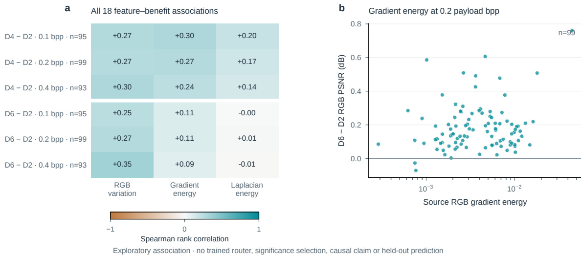
Figure S14. Cheap complexity measures do not directly identify the useful expert. All 18 specified feature/depth/rate combinations are shown, with supported image counts. The scatter panel was fixed to gradient energy versus D6-D2 at 0.2 bpp before inspecting the associations. These are correlations with interim equal-rate benefits, not router accuracy or causal feature effects.
