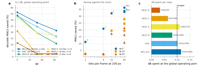
Figure 11. Saving by test class at one global operating point. \lambda is bisected once so the whole set lands on the budget, exactly as it would be in deployment; each class is then reported at that \lambda . The ordering follows tile count, not content.
