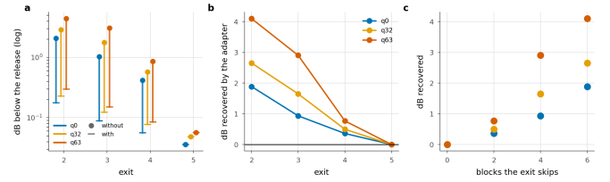
Figure 3. What the adapters are worth. a, each exit with and without its adapter. b, the dB the adapter recovers. c, the same against the number of blocks the exit skips — the design rationale, measured.
