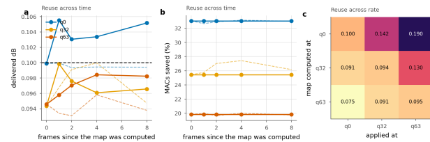
Figure 16. Reusing an exit map. Solid is the transferred map, dashed the one recomputed in place. a, b: reuse across frames of the same sequence. c: reuse across quality index; the entry is the delivered distortion against a 0.1 dB budget.
