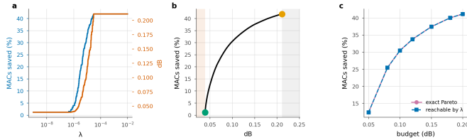
Figure 13. The structure of the allocation, on one frame. a , compute and distortion are monotone in the multiplier. b , the frontier between the floor (green) and saturation (orange); shaded regions are infeasible and wasted. c , what the Lagrangian reaches against the exact Pareto set, enumerated by dynamic programming — the two curves are indistinguishable.
