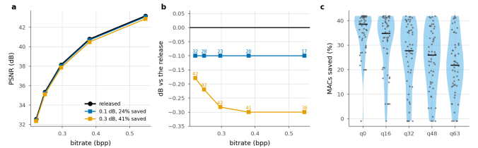
Figure 9. The plane a codec is read on, and the spread behind the mean. a , operating points against the released curve. b , the same with the quality axis expanded; labels are compute saved. c , per sequence at a matched point near 0.1 dB; one dot per sequence, bar is the median.
