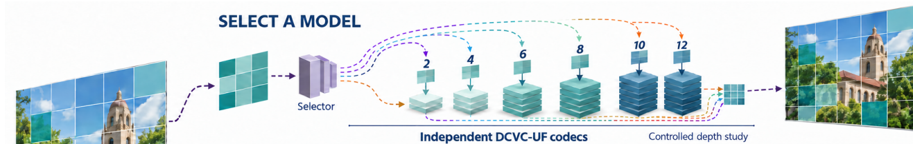
Figure 2. Independent-depth codec bank. A selector assigns a source region to one of six complete DCVC-UF codecs before encoding ; each depth learns its own analysis, entropy and synthesis transforms. Decoded regions are assembled into an image. This is a conceptual design under study, not a measured six-way router or an additional stage of the shared early-exit path in Fig. 3.
