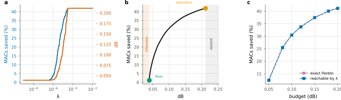
Figure 23. The structure of the allocation, on one frame. a, compute and distortion are monotone in the multiplier. b, the frontier, with both ends and both dead bands marked on the panel. c, what the Lagrangian reaches against the exact Pareto set, enumerated by dynamic programming.
