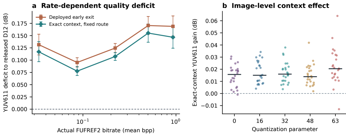
Figure S13. Kodak24 exact-context transfer at unchanged real bitrates. a , Mean YUV611 deficit to released D12 versus actual FUFREF2 bitrate for the deployed and diagnostic exact-context synthesis paths. Error bars are paired 24-image bootstrap 95% intervals; the released decoder is at zero deficit by definition. b , Per-image YUV611 gain from replacing zero-halo-plus-repair with clipped exact context and no repair, at each QP; dark bars mark medians. The exit maps remain fixed. No BD-rate or latency claim follows from this reconstruction-only counterfactual.
