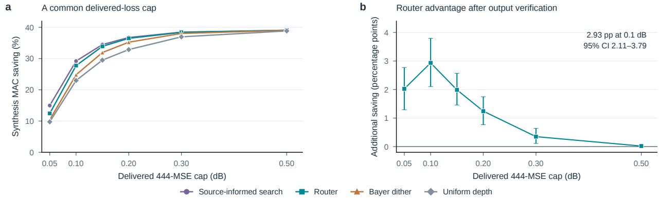
Figure 4. The spatial-routing margin survives a common measured quality cap. a , Lowest-cost eligible output within each policy’s recorded candidate pool. b , Paired router–dither saving and 95% sequence-cluster interval. Full-frame fallback is included in both panels. All 265 pairs remain in every comparison. This is retrospective selection among actual reconstructions, with fine-tuned e15 as the common anchor; candidate-acquisition time and released-reference quality are outside this five-QP analysis. A separate QP32 reference replay is reported in the supplement.
