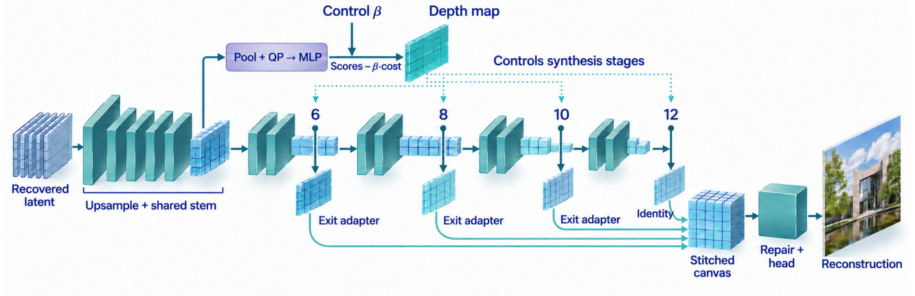
Figure 2. Share the representation; spend further depth only on surviving tiles. A four-block shared stem supplies the MLP with features and QP. Cost-adjusted scores select exits at total depths 6/8/10/12. Each departing feature passes through its adapter (identity at depth 12) into one canvas, followed by full-frame repair and reconstruction. The illustration follows the implemented connectivity; tensor contents and the output scene are conceptual, AI-generated artwork rather than measured reconstructions.
