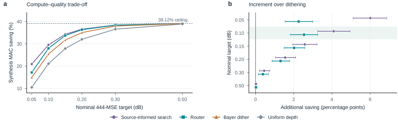
Figure 3. Early exit supplies the saving; spatial routing adds a budget-dependent margin. a , Modelled synthesis MAC reduction for four stopping rules. b , Paired advantages over Bayer dithering, with 95% sequence-cluster intervals; the shaded row highlights 0.1 dB. QP and fixed-cohort analyses are in the supplement. All curves use per-source calibration. MAC savings exclude router and signalling overhead and are not measured runtime reductions. Targets use the \Delta_{444} MSE-ratio loss defined in Sec. 3.
