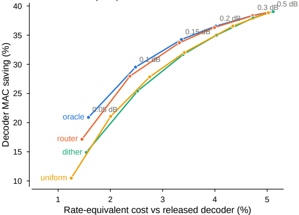
DCVC-UF: bits paid per MAC saved
