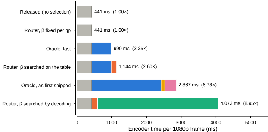
Encoder, 1920×1080, median of 210 frame-qp
