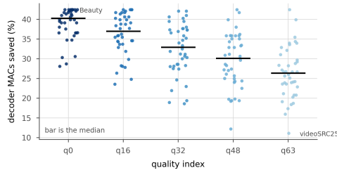
Figure 18. What the set mean hides. Every test sequence as a point, at the 0.1 dB budget; the bar is the median. At the lowest rate the saving runs from 28.1% to 42.5% across sequences and at the highest from 11.1% to 42.5%. The spread within a rate is larger than the difference between rates, and it is content, not noise: the same sequences sit at the same end of it at every rate.
