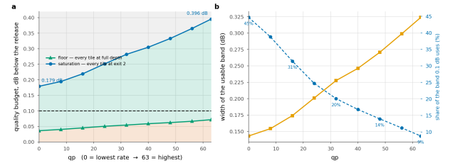
Figure 21. Three regions, and only the middle one is a design choice. Below the floor no allocation meets the budget; above saturation every tile already takes the cheapest exit. The 0.1 dB budget uses 45% of the band at the lowest rate and 9% at the highest.
