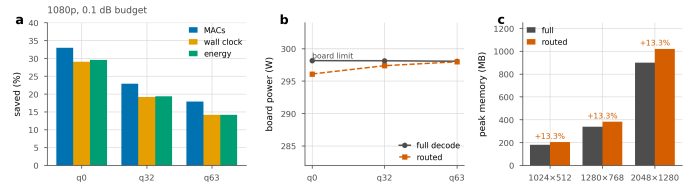
Figure 33. Three units for one saving. a, the same routed decode measured as arithmetic, as wall clock and as joules per frame, at 1080p and a 0.1 dB budget. Energy follows the clock, not the arithmetic. b, why: the board draws the same power either way, because the later groups run on a shrinking set of tiles and a partly idle GPU still draws its static power. c, peak memory, which routing raises rather than lowers, by 13.3% at every resolution that fitted on the card.
