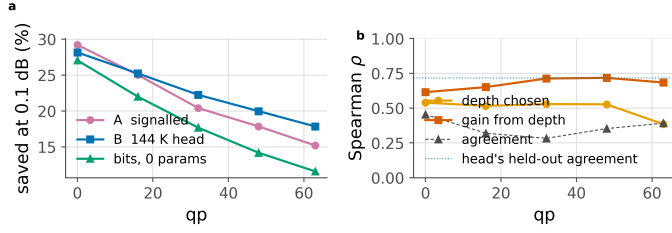
Figure 28. The calibrated bit rule. a , saving at 0.1 dB; shaded where the calibrated bit rule beats the trained head. b , what a tile’s bit count is correlated with, against how often the rule agrees with the oracle outright; dotted is the head’s own held-out agreement.
