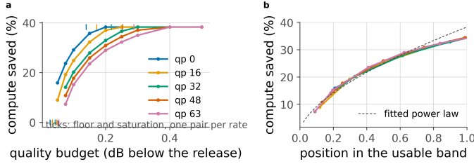
Figure 24. The band is the rate dependence. a , saving against the budget, with each rate's floor and saturation point ticked. b , the same with the budget axis rescaled onto each rate's own band. Five curves become one; dashed is the one-parameter power law fitted to all of them.
