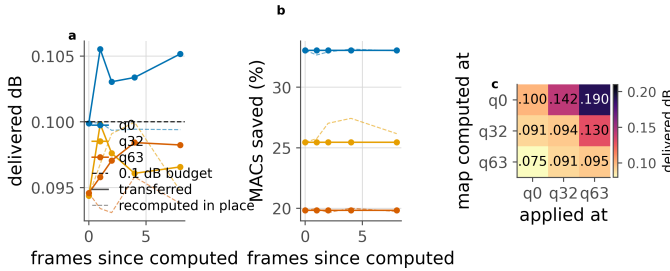
Figure 34. Reusing an exit map. Solid is the transferred map, dashed the one recomputed in place. a, b: reuse across frames of the same sequence. c: reuse across quality index; the entry is the delivered distortion against a 0.1 dB budget.
