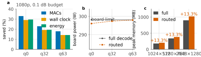
Figure 35. Three units for one saving. a, the same routed decode measured as arithmetic, as wall clock and as joules per frame, at 1080p and a 0.1 dB budget. Energy follows the clock, not the arithmetic. b, why: the board draws the same power either way, because the later groups run on a shrinking set of tiles and a partly idle GPU still draws its static power. c, peak memory, which routing raises rather than lowers, by 13.3% at every resolution that fitted on the card.
