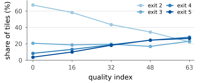
Figure 5. Where the tiles actually go, at the 0.1 dB budget, pooled over the whole test set: the share of tiles taking each exit, against rate. Exits below the split depth are not drawn because a tile cannot take one. At the lowest rate two thirds of tiles take the cheapest available exit; at the highest only a fifth do and a quarter need the deepest. The allocation is not degenerate at either end, which is what makes the choice worth making.
