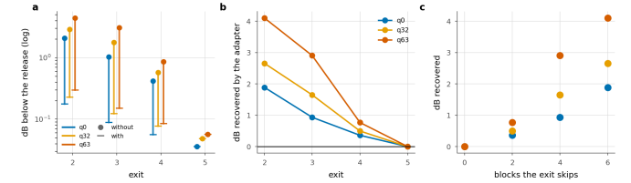
Figure 4. What the adapters are worth. a, each exit with and without its adapter. b, the dB the adapter recovers. c, the same against the number of blocks the exit skips — the design rationale, measured.
