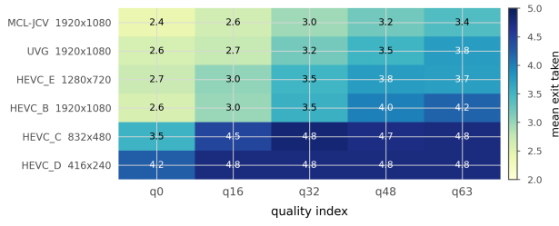
Figure 21. How deep each class has to go. Mean exit taken by the tiles of each test class at the 0.1 dB budget, ordered by that mean. Resolution is the strongest predictor: the 416×240 class has two tiles a frame and almost no choice, and the 1080p classes have forty and use the whole ladder. This is the dependence Section 5.3 measures, seen per class rather than pooled.
