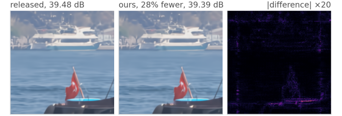
Figure 30. What 28.1% of the arithmetic costs, to look at. Bosphorus at q32, one frame, with \lambda bisected on that frame to 0.100 dB. Both crops are decoded from the same latent at 0.2740 bpp: the released decoder reaches 39.48 dB and the routed decode 39.39 dB. The crop is centred on the tile that gave up the most, tile 18 of 40, not on a flattering one. Right, the absolute difference at \times 20 .
