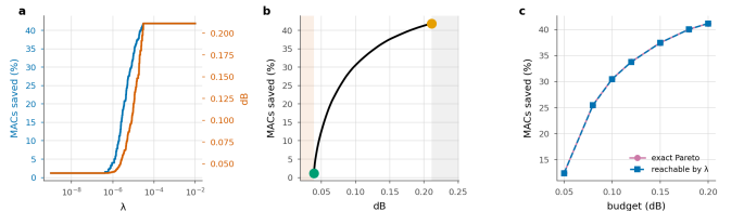
Figure 22. The structure of the allocation , on one frame. a , compute and distortion are monotone in the multiplier. b , the frontier between floor and saturation; shaded regions are infeasible or wasted. c , what the Lagrangian reaches against the exact Pareto set, enumerated by dynamic programming.
