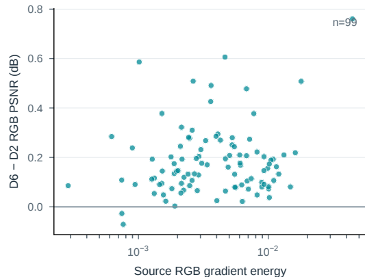
b Gradient energy at 0.2 payload bpp
