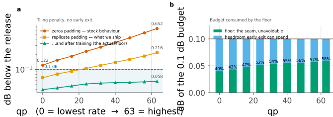
Figure 52. The tiling penalty across the whole rate range, every tile at full depth, so this is the floor and nothing else. a, the steps that reduce it, of which the two that matter cost no arithmetic; the largest single factor is training the ladder with the seam present. b, the floor as a share of the 0.1 dB budget: it is charged inside the budget and consumes a growing part of it as the rate rises, which is one of the two reasons the saving falls with rate.
