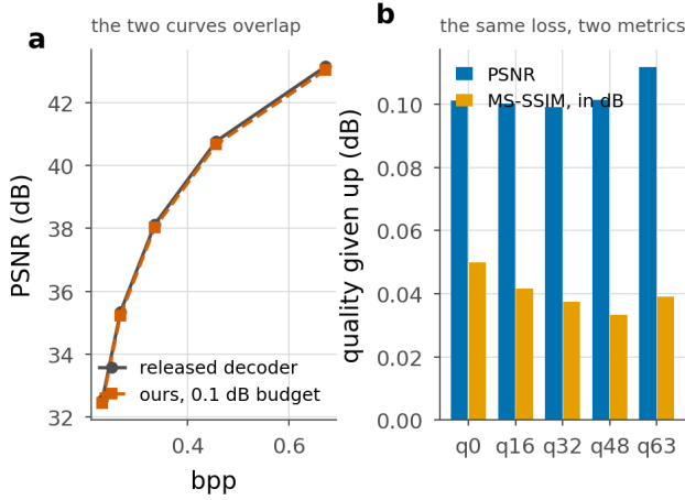
Figure 45. a , the rate-quality curve of the released decoder and of ours at the 0.1 dB budget, over the five quality indices. At plot scale they are one curve, which is what a 0.1 dB budget means. b , the gap that panel a cannot show, in PSNR and in MS-SSIM expressed as a decibel.
