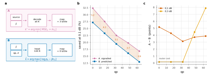
Figure 14. Who decides. (a) A holds the source, so it can decode all K exits per tile and pick the true minimiser; it signals the map at \sim 90 bits/frame. B never sees the source — a 144 K-parameter head reads \hat{y} -hat, the entropy scales and qp — and signals nothing. (b) Saving at 0.1 dB; shading is what a bit-exact bitstream costs. (c) That cost is smallest at q32, where the tilt needed to move the router off its training multiplier is essentially zero, and grows in both directions. At 0.3 dB it collapses to the router's own 0.163% wherever the budget saturates the ladder, and widens where it does not.
