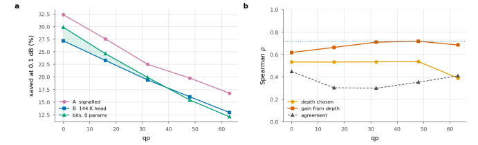
Figure 15. The free baseline. a Saving at 0.1 dB; shaded where the parameter-free rule beats the trained head. b What a tile's bit count is correlated with, against how often the rule agrees with the oracle outright; dotted is the head's own held-out agreement.
