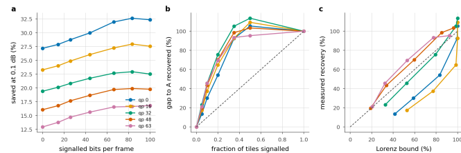
Figure 16. Partial signalling. a Saving against the bits spent on the map; the left end of each line is B and the right end is A. b The same, normalised: what fraction of the A–B gap a given fraction of the map recovers; above 100% a partial map is
