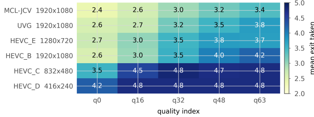
Figure 19. How deep each class has to go. Mean exit taken by the tiles of each test class at the 0.1 dB budget, ordered by that mean. Resolution is the strongest predictor: the 416×240 class has two tiles a frame and almost no choice, and the 1080p classes have forty and use the whole ladder. This is the dependence Section 5.3 measures, seen per class rather than pooled.
