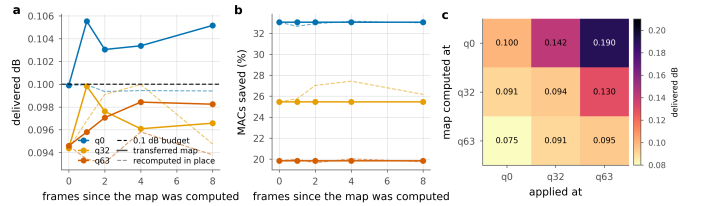
Figure 34. Reusing an exit map. Solid is the transferred map, dashed the one recomputed in place. a , b : reuse across frames of the same sequence. c : reuse across quality index; the entry is the delivered distortion against a 0.1 dB budget.
