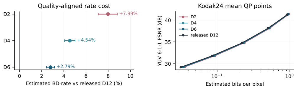
Figure S15. The completed independent codecs approach the release as depth grows. Left, per-image YUV 6:1:1 BD-rate cost on the four-model common PSNR interval; bars are 95% paired-image bootstrap intervals ( n = 24 ). Right, mean five-QP operating points on Kodak24. Rates are deterministic entropy estimates, not actual bitstreams. Released D12 differs in training history from the three scratch models.
