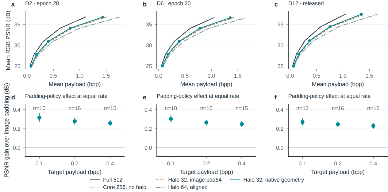
Figure S31. Keep spatial rounding inside the codec contract. a–c , Actual-payload RD points averaged over the fixed 16-image cohort, with shared axis limits. d–f , Per-image matched-rate gain from moving padding to the latent, with paired 95% image-bootstrap intervals. Each rate uses the common support of all five variants within that depth; n denotes supported images out of 16, with no extrapolation. The latent-padding implementation uses CPU FP32 research streams; “native geometry” does not denote native CUDA output or latency.
