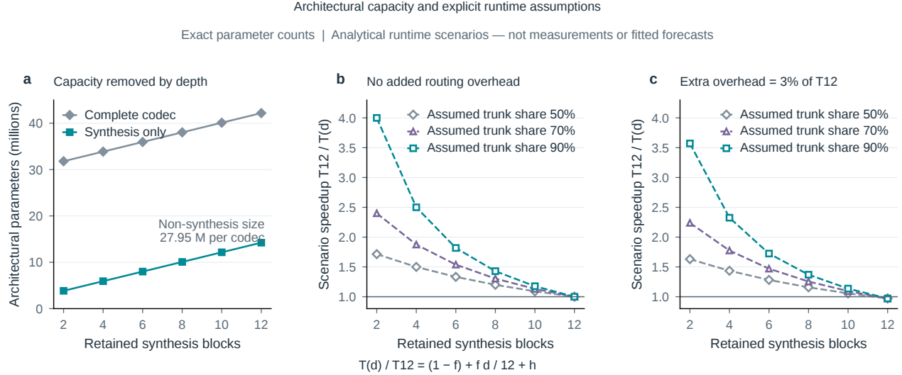
Figure S23. A transparent design-space illustration for unfinished experiments. a , Exact architectural parameter counts. b,c , Analytical runtime sensitivity to assumed trunk-time share and added overhead. Open markers and dashed lines denote assumptions, not measurements or fitted forecasts. No quality or bitrate outcome is assigned to an unfinished model.
