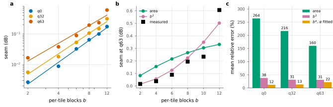
Figure 62. The seam against per-tile depth. a, the measurement with the fitted power law. b, both models against q63, one free scale each. c, mean relative error. The area fraction saturates once the border reaches every pixel and the penalty does not, which is where the area law fails as a predictor.
