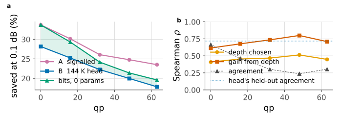
Figure 28. The calibrated bit rule. a, saving at 0.1 dB; shaded where the calibrated bit rule beats the trained head. b, what a tile's bit count is correlated with, against how often the rule agrees with the oracle outright; dotted is the head's own held-out agreement.
