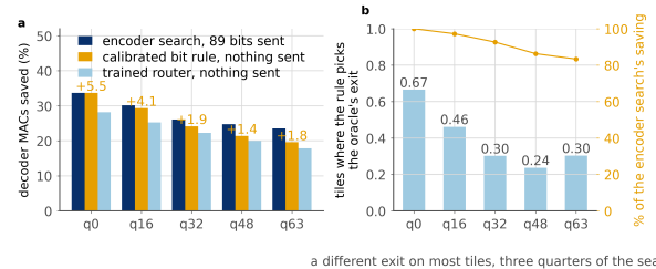
Figure 30. Three ways to choose an exit. a, saving at 0.1 dB. The encoder search sees the source and sends 89 bits a frame; the other two send nothing. The bit rule beats the trained head at every rate, with no learned parameters against the head's 144,030. b, bars are the tiles where the rule picks the search's exit, the line the fraction of its saving it captures anyway.
