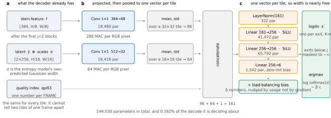
Figure 10. The router head. a , the three things it reads, all already held by the decoder. b , each projected by a 1×1, then reduced to one vector per tile by its mean and standard deviation. c , a three-layer perceptron, one pass per tile. Every shape and parameter count is read off the module when the figure is drawn.
