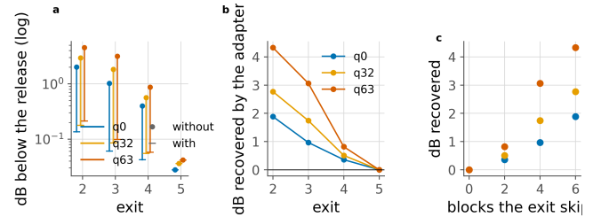
Figure 8. What the adapters are worth. a , each exit with and without its adapter. b , the dB the adapter recovers. c , the same against the number of blocks the exit skips, which is the design rationale measured.
