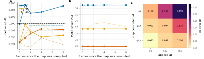
Figure 33. Reusing an exit map. Solid is the transferred map, dashed the one recomputed in place. a , b : reuse across frames of the same sequence. c : reuse across quality index; the entry is the delivered distortion against a 0.1 dB budget.
