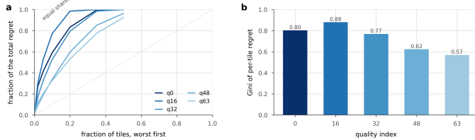
Figure 32. The loss is concentrated. a , the share of the total regret carried by the worst fraction of tiles, per rate; the dotted line is what an even spread would look like. b , the same as a small minority of tiles carries most of what staying silent costs, which is why signalling a fraction of the map recovers most of the gap.
