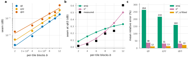
Figure 12. The seam against per-tile depth. a , the measurement with the fitted power law. b , both models against q_{63} , one free scale each. c , mean relative error. The area fraction saturates once the border reaches every pixel; the penalty does not.
