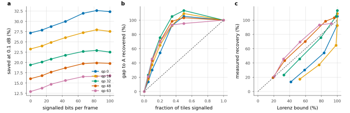
Figure 18. Partial signalling. a Saving against the bits spent on the map; the left end of each line is B and the right end is A. b The same, normalised: what fraction of the A–B gap a given fraction of the map recovers; dashed is proportional recovery, and above 100% a partial map is beating a complete one. c The same against the fixed- \lambda Lorenz prediction; dashed is equality, and points above it are allocations a single multiplier cannot reach.
