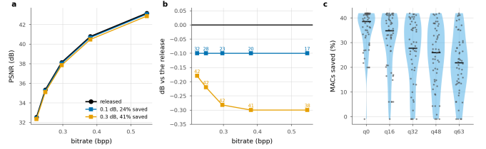
Figure 9. The plane a codec is read on, and the spread behind the mean. a , operating points against the released curve. b , the same with the quality axis expanded; labels are compute saved. c , per sequence at a matched point near 0.1 dB; one dot per sequence, bar is the median.
