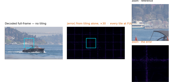
Figure 4. The artefact, before anything is done about it. One frame decoded twice from the same bitstream with the same weights, every tile at full depth, stock zero padding, and no early exit anywhere. The only difference is that the right-hand decode was tiled. The error map is the tile lattice and nothing else.
