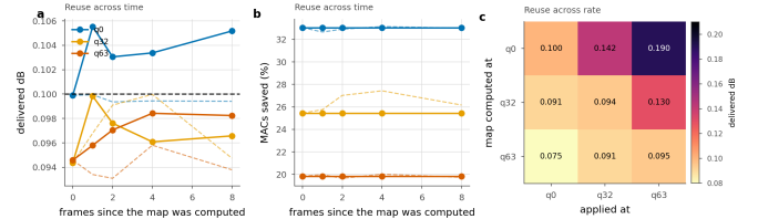
Figure 14. Reusing an exit map. Solid is the transferred map, dashed the one recomputed in place. a, b : reuse across frames of the same sequence. c : reuse across quality index; the entry is the delivered distortion against a 0.1 dB budget.
