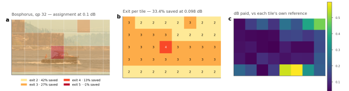
Figure 10. Where the decoder spends. (a) the assignment overlaid on the frame, (b) the exit index per tile, (c) the quality each tile gives up against its own full-depth reference. Water and sky leave at the shallowest rung; the boat and shoreline run deep.
