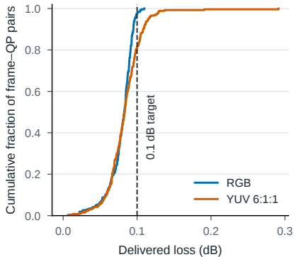
b A target is not a framewise guarantee
