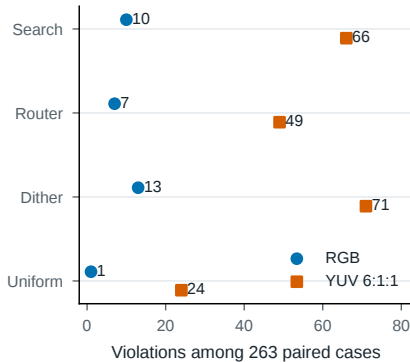
c Count violations in the output metric
