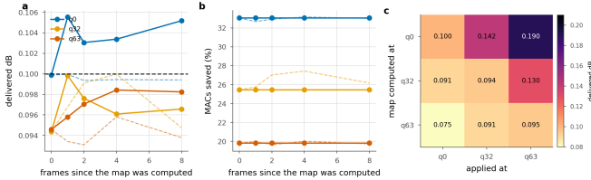
Figure 18. Reusing an exit map. Solid is the transferred map, dashed the one recomputed in place. a, b: reuse across frames of the same sequence. c: reuse across quality index; the entry is the delivered distortion against a 0.1 dB budget.
