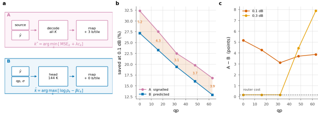
Figure 15. Who decides. (a) A holds the source, so it can decode all K exits per tile and pick the true minimiser; it signals the map at ~90 bits/frame. B never sees the source — a 144 K-parameter head reads \hat{y} , the entropy scales and qp — and signals nothing. (b) Saving at 0.1 dB; shading is what a bit-exact bitstream costs and qp — and signals nothing. (c) That cost is smallest at q32, where the tilt needed to move the router off its training multiplier is essentially zero, and grows in both directions. At 0.3 dB it collapses to the router's own 0.163% wherever the budget saturates the ladder, and widens where it does not.
