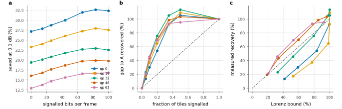
Figure 17. Partial signalling. a Saving against the bits spent on the map; the left end of each line is B and the right end is A. b The same, normalised: what fraction of the A–B gap a given fraction of the map recovers; above 100% a partial map is beating a complete one. c The same against the fixed- \lambda Lorenz prediction; dashed is equality, and points above it are allocations a single multiplier cannot reach.
