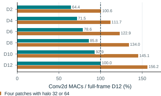
d Encoder with reconstruction
