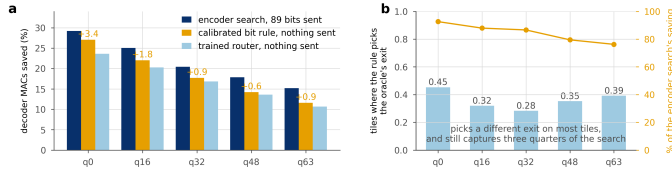
Figure 30. Three ways to choose an exit. a, saving at 0.1 dB. The encoder search sees the source and sends 89 bits a frame; the other two send nothing. The bit rule beats the trained head at every rate, with no learned parameters against the head's 144,030. b, bars are the tiles where the rule picks the search's exit, the line the fraction of its saving it captures anyway.
