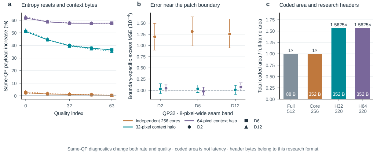
Figure S21. A better seam and a better codec are different outcomes. a , Same-QP payload increase over the full-frame model. b , At QP32, patch-minus-full MSE in the central 8-pixel seam band, minus the corresponding interior excess. c , Exact coded area and research-header bytes. Halo32 and halo64 have equal coded area under this padding policy, but different real context. Area ratios are not latency ratios, and same-QP seam diagnostics are not equal-rate quality comparisons.
