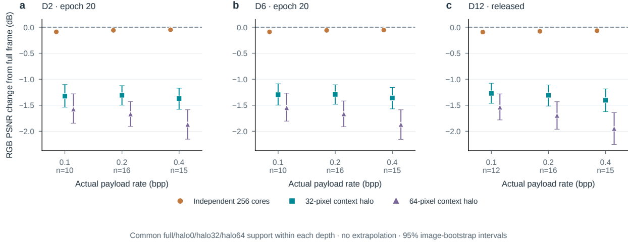
Figure S20. Charge repeated context to the transmitted rate. RGB PSNR changes from the same full-frame model at matched actual payload rate. Each depth uses the common supported images across full frame and all three patch variants; counts are shown and the vertical scale is shared. Intervals resample paired images. D2/D6 are interim epoch 20 models; D12 has different released training provenance. The experiment holds depth fixed within every contrast and makes no adaptive-routing or runtime claim.
