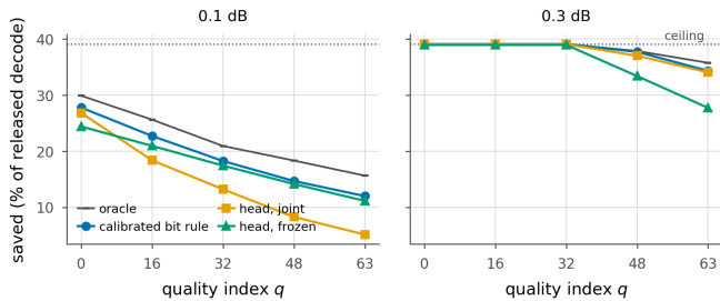
Figure 29. The rule sits between the two heads and the oracle. Saving at each rate, against the Lagrangian oracle measured inside the same run and the architectural ceiling (dotted). At 0.1 dB the rule is above both heads at every rate, and the gap between the two heads is wider than the gap between the rule and either of them. At 0.3 dB the three lowest rates saturate and the three curves separate only at q48 and q63.
