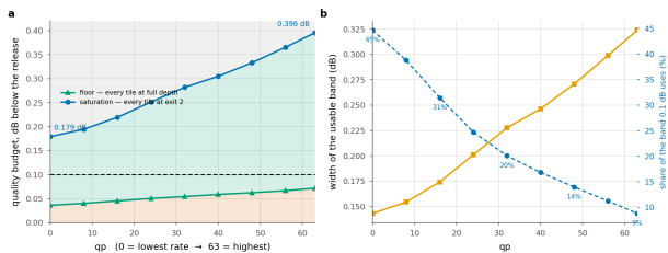
Figure 22. Three regions, and only the middle one is a design choice. Below the floor no allocation meets the budget; above saturation every tile already takes the cheapest exit and a looser budget buys nothing. The 0.1 dB budget uses 45% of the band at the lowest rate and 9% at the highest, which is why the same budget behaves so differently at the two ends of the rate range.
