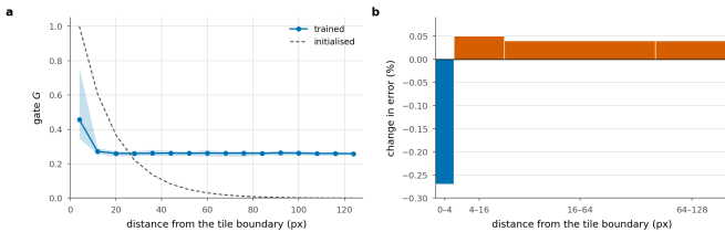
Figure 34. The learned deblocking filter, and where it wins. It is gated by position within a tile and applied once to the stitched frame, for 1.09% of the decode. a , the trained gate against distance from the boundary, beside its initialisation. b , the change in error by that distance; bar width is the share of pixels, so bar area is the contribution to the frame. It wins on the pixels nearest a boundary and loses on the rest, which is why a perfect gate still cannot pay for it.
