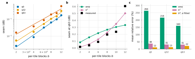
Figure 35. The seam against per-tile depth. a , the measurement with the fitted power law. b , both models against q63, one free scale each. c , mean relative error. The area fraction saturates once the border reaches every pixel and the penalty does not, which is where the area law fails as a predictor.
