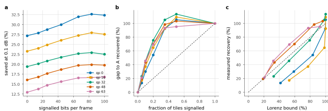
Figure 30. Partial signalling, drawn. a , saving against the bits spent on the map; each line runs from configuration B on the left to configuration A on the right. b , the same normalised by the A-to-B gap, with proportional recovery dashed. c , against the fixed-multiplier Lorenz bound of C.7; points above the dashed line are allocations one multiplier cannot reach.
