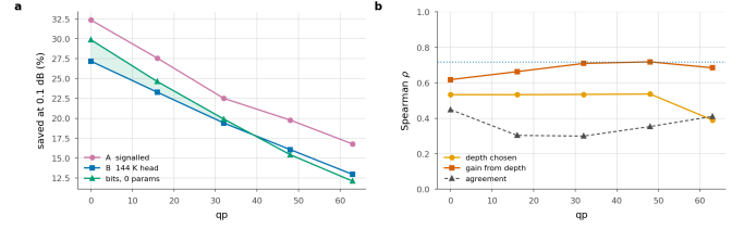
Figure 7. The calibrated bit rule. a Saving at 0.1 dB; shaded where the calibrated bit rule beats the trained head. b What a tile's bit count is correlated with, against how often the rule agrees with the oracle outright; dotted is the head's own held-out agreement.
