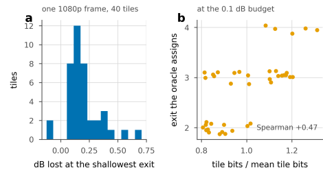
Figure 2. Why depth should not be uniform. One 1080p frame, 40 tiles. a , what each tile loses if it stops at the shallowest exit the ladder allows: several lose nothing measurable and the worst loses several times the budget, so a single depth for the frame has to be set by the worst of them. b , the bits the entropy model has already spent on a tile against the exit the Lagrangian oracle sends it to, at the 0.1 dB budget. The signal a decoder-side router needs is already in the file.
