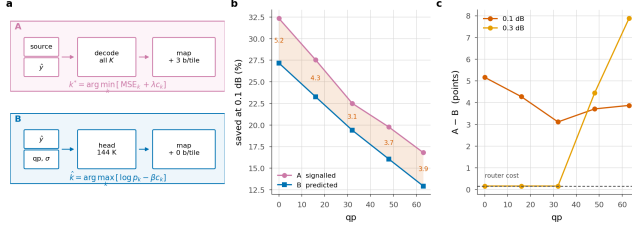
Figure 6. Who decides. a , the two decision paths side by side: the encoder's search over all K exits per tile against the head's forward pass over decoded data. b , saving at 0.1 dB; shading is what a bit-exact bitstream costs. c , that cost is smallest at q32, where the router needs almost no cost multiplier to reach the budget from where it was trained, and grows in both directions. At 0.3 dB it falls to the router's own 0.163% wherever the budget saturates the ladder, and widens where it does not.
