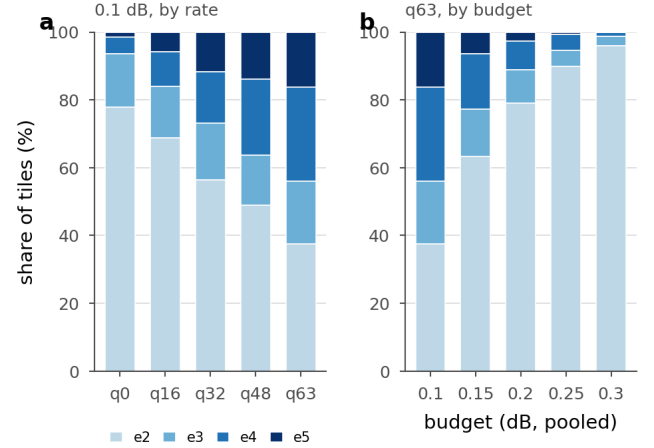
Figure 17. How the ladder fills up. a , exit shares at the 0.1 dB budget as the rate rises. b , exit shares at q63 as the budget loosens, until at 0.3 dB 96% of tiles are already at the shallowest exit and there is almost nothing left to allocate. Both panels are pooled over the test set.
