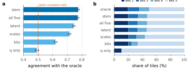
Figure 27. The input ablation, both halves of it. a , agreement with the oracle per variant, with one standard error across frames; the dashed line is the best single constant exit. The two dark bars are the two heads that see the stem. b , where each variant sends its tiles, against the oracle's own distribution. Every variant reproduces the oracle's use of the shallowest exit to within a point, and what degrades as inputs are removed is the separation of the middle of the ladder: the bit count alone nearly empties exit 3, and q alone uses two of the four exits available to it.
