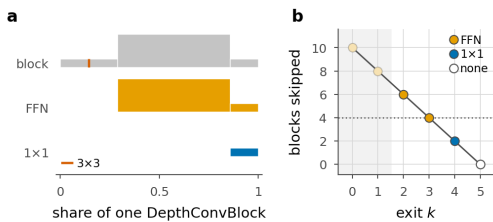
Figure 9. Inside an exit adapter. a , one DepthConvBlock and the two adapters, drawn to scale: bar length is a share of the block, bar height the channel width written. Neither adapter contains the block's only 3×3 (the hairline rule), so neither adds receptive field or seam penalty, which is the design constraint the seam measurement imposes. b , blocks skipped per exit, coloured by adapter; the rule switches to the FFN at four skipped blocks. Lengths are counted with hooks off the modules themselves.
