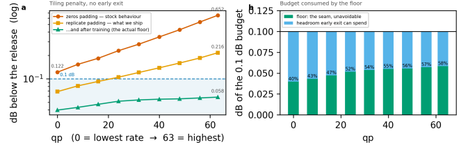
Figure 23. The tiling penalty across the whole rate range, every tile at full depth, so this is the floor and nothing else. a , the steps that reduce it, of which the two that matter cost no arithmetic; the largest single factor is training the ladder with the seam present. b , the floor as a share of the 0.1 dB budget: it is charged inside the budget and consumes a growing part of it as the rate rises, which is one of the two reasons the saving falls with rate.
