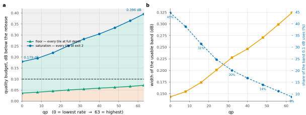
Figure 22. Three regions, and only the middle one is a design choice. Below the floor no allocation meets the budget; above saturation every tile already takes the cheapest exit and a looser budget buys nothing. The 0.1 dB budget uses 45% of the band at the lowest rate and 9% at the highest, which is why the same budget behaves so differently at the two ends of the rate range.
