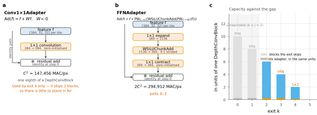
Figure 2. Inside an exit adapter. Both kinds are entirely pointwise, so no adapter adds receptive field and none contributes any tile-boundary penalty. Capacity is matched to the number of blocks the exit skips, and charged for: an exit-2 tile saves six blocks minus 0.25, not six.
