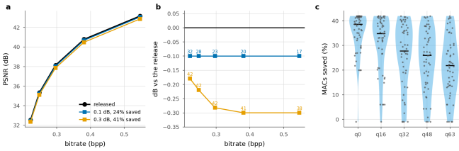
Figure 8. The plane a codec is read on, and the spread behind the mean. a , operating points against the released curve. b , the same with the quality axis expanded; labels are compute saved. c , per sequence at a matched point near 0.1 dB; one dot per sequence, bar is the median.
