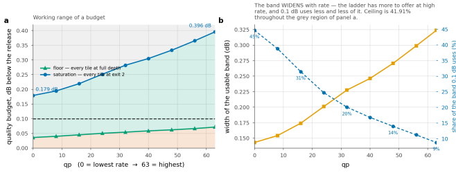
Figure 11. Three regions, and only the middle one is a design choice. Below the floor no allocation meets the budget; above saturation every tile is already on the cheapest rung. The working 0.1 dB budget uses 45% of the window at the lowest rate and 9% at the highest.
