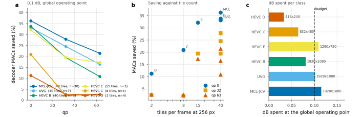
Figure 10. Saving by test class at one global operating point. \lambda is bisected once so the whole set lands on the budget, exactly as it would be in deployment; each class is then reported at that \lambda . The ordering follows tile count, not content.
