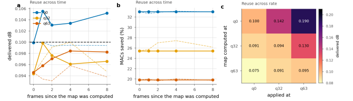
Figure 14. Reusing an exit map. Solid is the transferred map, dashed the one recomputed in place. a , b : reuse across frames of the same sequence. c : reuse across quality index; the entry is the delivered distortion against a 0.1 dB budget.
