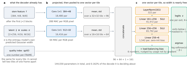
Figure 10. The router head. a, the three things it reads, all already held by the decoder. b, each projected by a 1 \times 1 , then reduced to one vector per tile by its mean and standard deviation. c, a three-layer perceptron, one pass per tile. Every shape and parameter count is read off the module when the figure is drawn.
