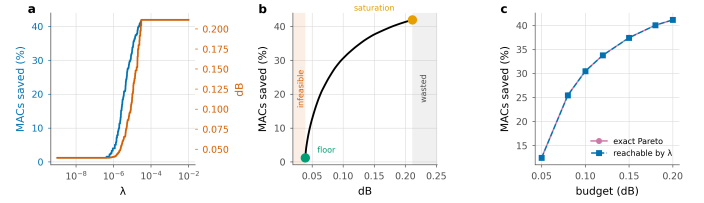
Figure 23. The structure of the allocation , on one frame. a , compute and distortion are monotone in the multiplier. b , the frontier, with both ends and both dead bands marked on the panel. c , what the Lagrangian reaches against the exact Pareto set, enumerated by dynamic programming.
