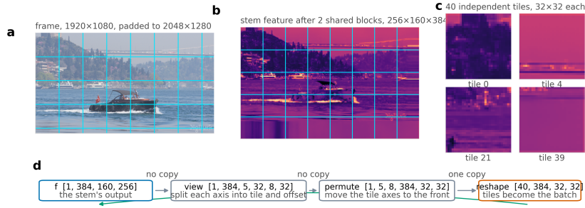
Figure 6. What patchify does. From one real decode. a , the frame padded to whole tiles, with the grid the decoder will impose. b , the feature map after the shared stem at one eighth resolution, so a 256 px tile is 32 \times 32 of features: the tiling happens here, not in the pixel domain. c , four of the 40 tiles as the trunk sees them. d , the operation and its inverse, which costs no arithmetic and is exact.
