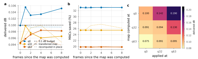
Figure 34. Reusing an exit map. Solid is the transferred map, dashed the one recomputed in place. a , b : reuse across frames of the same sequence. c : reuse across quality index; the entry is the delivered distortion against a 0.1 dB budget.
