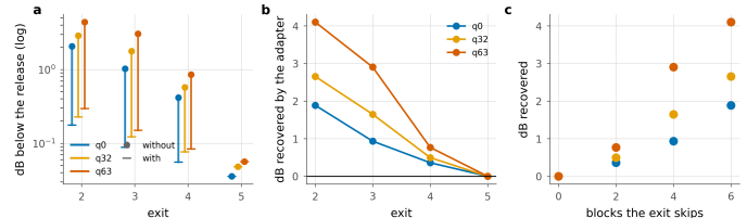
Figure 8. What the adapters are worth. a , each exit with and without its adapter. b , the dB the adapter recovers. c , the same against the number of blocks the exit skips, which is the design rationale measured.
