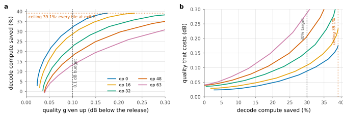
Figure 25. The trade-off, whole. a , what a budget buys, per rate; the dotted line is the arithmetic ceiling, 39.1%, and q0 reaches it at 0.179 dB. b , the same relation inverted, so it reads as what a saving target costs. The three budgets reported elsewhere are three points on this curve.
