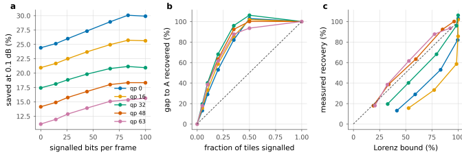
Figure 32. Partial signalling. a , saving against the bits spent on the map; each line runs from B on the left to A on the right. b , the same normalised by the A-to-B gap; dashed is proportional recovery. c , against the fixed- \lambda Lorenz bound; points above the dashed line are allocations one multiplier cannot reach.
