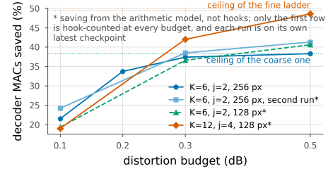
Figure 33. The right ladder depends on the budget. Saving against budget for four ladders, with each one's architectural ceiling as a dotted line. A finer ladder has a higher ceiling and a higher floor, so the curves cross: the coarse ladder wins where the budget is tight and cannot be spent, and the fine one wins where it is loose enough to reach exits the coarse ladder does not have. The crossing is the design choice this section is about.
