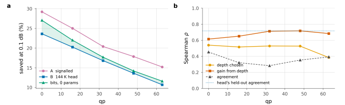
Figure 28. The calibrated bit rule. a , saving at 0.1 dB; shaded where the calibrated bit rule beats the trained head. b , what a tile's bit count is correlated with, against how often the rule agrees with the oracle outright; dotted is the head's own held-out agreement.
