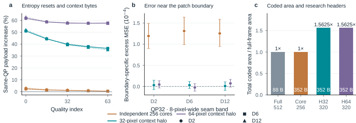
Figure S27. A better seam and a better codec are different outcomes. a , Same-QP payload increase over the full-frame model. b , At QP32, patch-minus-full MSE in the central 8-pixel seam band, minus the corresponding interior excess. c , Exact coded area and research-header bytes. Halo32 and halo64 have equal coded area under this padding policy, but different real context. Area ratios are not latency ratios, and same-QP seam diagnostics are not equal-rate quality comparisons.
