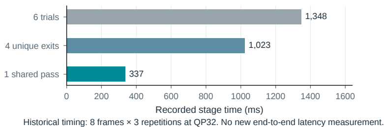
Figure S22. The decision path has an encoder cost. a , Stages required for source-error-based selection, with prefix reuse across candidate exits. b , Historical table-construction upper medians over 24 pooled trials, without invented uncertainty bars. c , A fixed held-out control and per-frame source calibration require different information. This is a stage analysis, not an end-to-end speedup.
