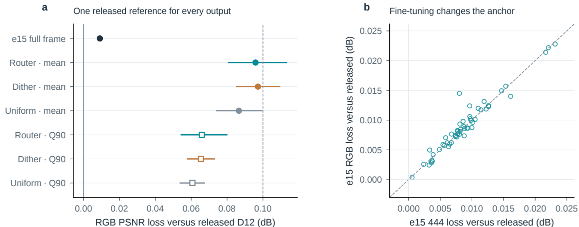
Figure S24. Measure the anchor before interpreting the loss budget. The same 53 first frames, QP32, valid-pixel support and CPU FP32 reconstruction. a , e15 full-frame and six fixed policies relative to released D12; points and intervals show means and paired 95% sequence-bootstrap intervals. Filled circles use mean control and hollow squares Q90; the dark full-frame point measures anchor drift. The dashed 0.1 dB line is a numerical reference. b , Per-sequence e15 drift under equal-channel unclipped 444 and converted/clipped RGB. The diagonal denotes metric agreement. No output or policy is reselected when the reference changes.
