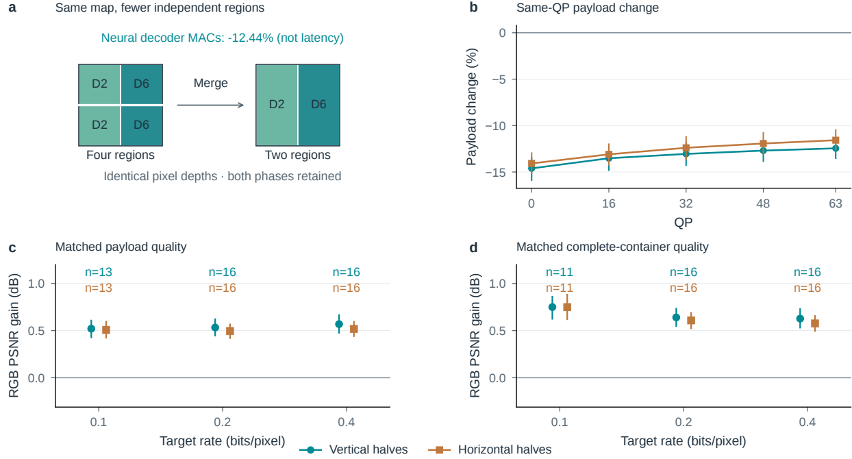
Figure S30. Better region execution without a better selector. a , One phase of the fixed depth-map control; every pixel keeps its D2 or D6 assignment. b , Same-QP relative payload change after coalescing. c,d , RGB PSNR gain at matched payload and complete-container rate, on shared vertical scales. Complementary phases are averaged within image before 95% paired-image bootstrap intervals. Counts show the common support of both phases and implementations, without extrapolation. The 800 outputs include unmerged checkerboards; those have no adjacent same-depth regions to combine. CPU FP32 research streams and epoch-20 weights are used throughout; this is neither learned routing nor a runtime benchmark.
