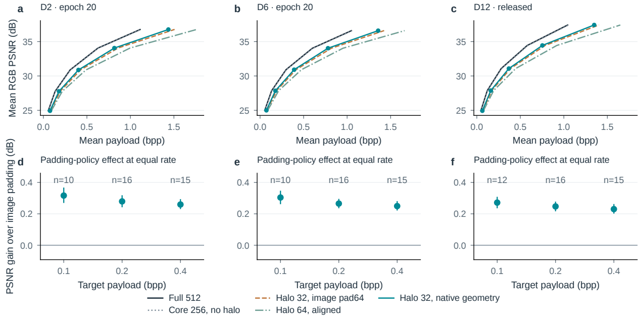
Figure S29. Keep spatial rounding inside the codec contract. a–c , Actual-payload RD points averaged over the fixed 16-image cohort, with shared axis limits. d–f , Per-image matched-rate gain from moving padding to the latent, with paired 95% image-bootstrap intervals. Each rate uses the common support of all five variants within that depth; n denotes supported images out of 16, with no extrapolation. The latent-padding implementation uses CPU FP32 research streams; “native geometry” does not denote native CUDA output or latency.
