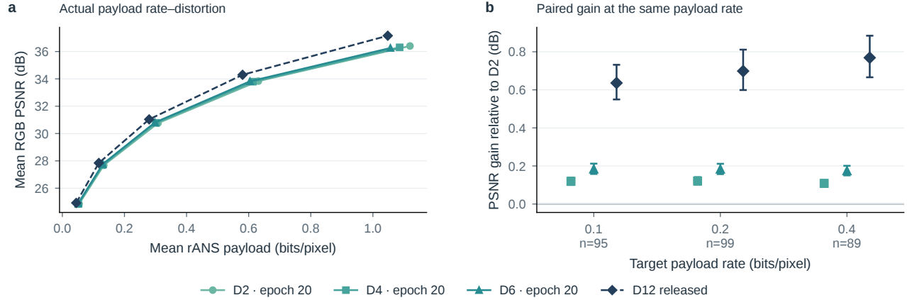
Figure S15. Shallow models are close, but not identical, at equal coded rate. a , Mean RGB PSNR and actual payload over all 100 crops at five QPs; joining lines are visual guides. b , Per-image interpolation and paired differences on four-model common support, with 95% image-bootstrap intervals. D2/D4/D6 are frozen epoch-20 models; released D12 is not matched in training history. These measured streams establish an interim CPU rate–distortion comparison, not final quality or native runtime.
