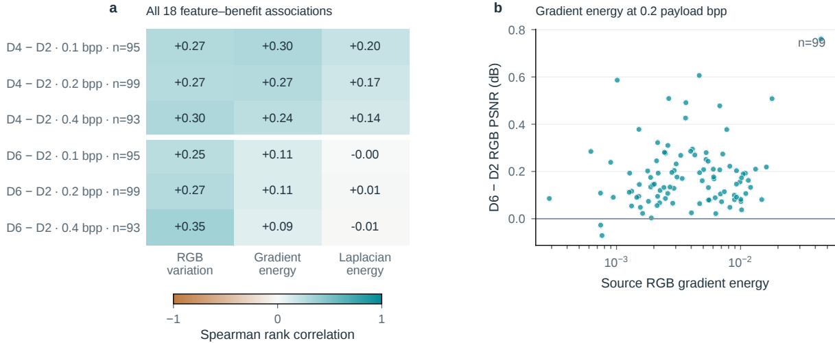
Figure S20. Cheap complexity measures do not directly identify the useful expert. All 18 specified feature/depth/rate combinations are shown, with supported image counts. The scatter panel was fixed to gradient energy versus D6–D2 at 0.2 bpp before inspecting the associations. These are correlations with interim equal-rate benefits, not router accuracy or causal feature effects.
