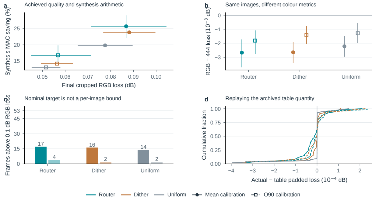
Figure S23. Carry the fixed decision through to the actual image. All 53 sequences at QP32, with no outcome-based exclusions. a , Achieved RGB loss and synthesis MAC saving with conditional 95% sequence-bootstrap intervals; these points are not an equal-quality frontier. b , RGB-minus-444 loss on the same support and reference. c , Counts above the nominal numerical threshold; pale bars denote Q90 calibration. d , Actual-minus-table loss on padded support. Mean and Q90 controls use a different calibration reference and metric from the cropped RGB report. The paired router-dither saving intervals include zero under both controls.
