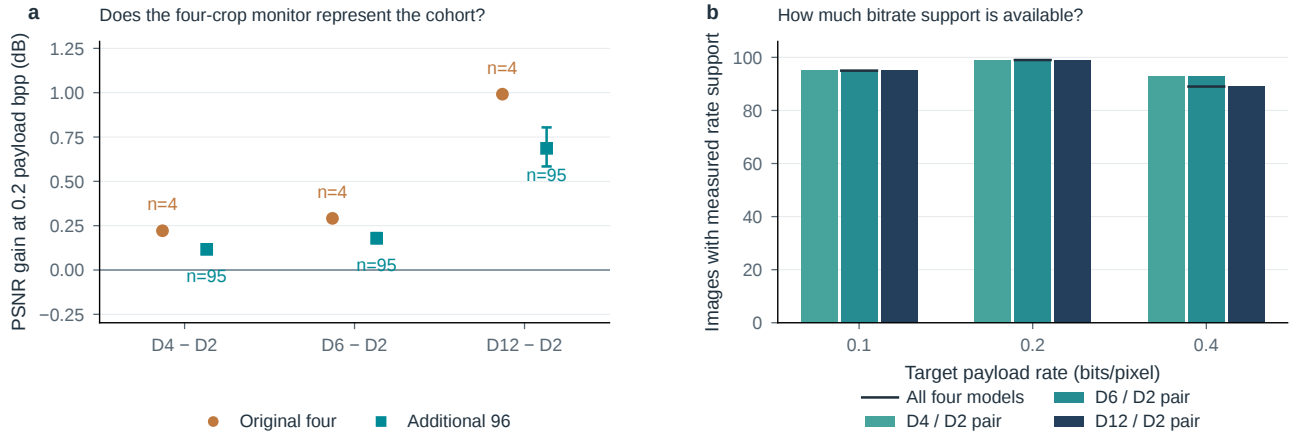
Figure S16. Coverage is part of the result. a , Original monitor crops and additional images at 0.2 payload bpp, restricted to four-model common support. We do not estimate uncertainty from the four-crop subset. b , Pairwise and four-model supported counts at each target rate. A changing cohort is made explicit rather than filled by extrapolation.
