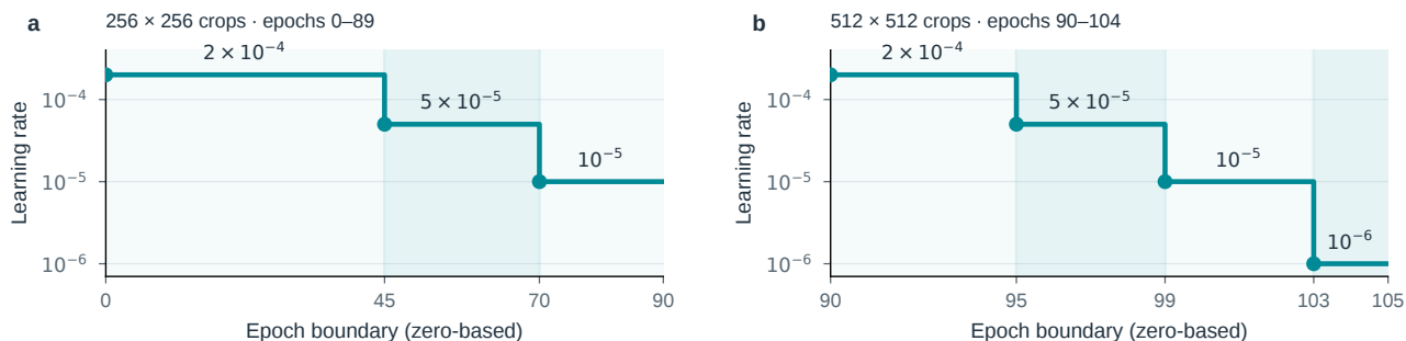
Figure S12. The full official schedule is retained. a , First 90 epochs with 256^2 crops. b , Final 15 epochs with 512^2 crops, on a separately expanded epoch axis. Zero-based boundaries delimit the seven learning-rate stages; the protocol applies to D2/D4/D6. These are prescribed settings, not learning curves.
