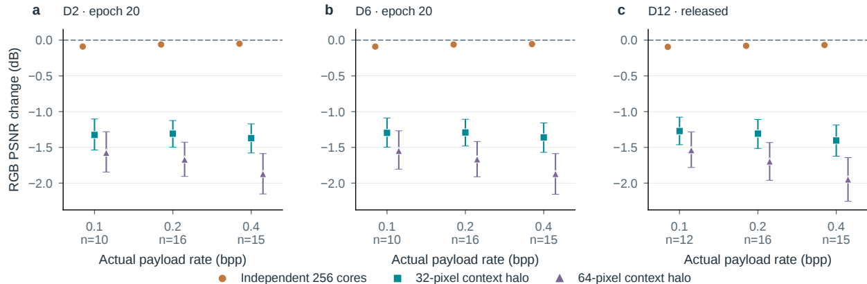
Figure S26. Charge repeated context to the transmitted rate. RGB PSNR changes from the same full-frame model at matched actual payload rate. Each depth uses the common supported images across full frame and all three patch variants; counts are shown and the vertical scale is shared. Intervals resample paired images. D2/D6 are interim epoch 20 models; D12 has different released training provenance. The experiment holds depth fixed within every contrast and makes no adaptive-routing or runtime claim.
