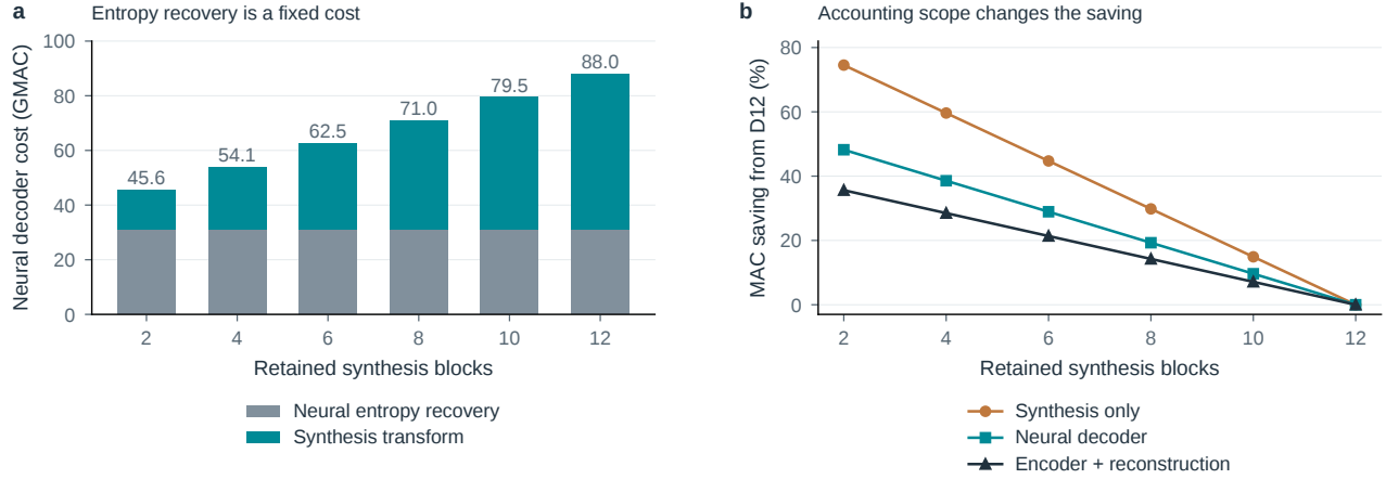
Figure S14. The arithmetic denominator changes the apparent saving. a , Synthesis varies with depth while neural entropy recovery stays fixed. b , The same architectural intervention under three accounting scopes. Counts use 512 \times 512 input and one MAC per multiply-accumulate; they are not observed kernel times. D8/D10 are architecture-only controls. Encoder totals include reconstruction but omit rANS, elementwise work, transfers and control overhead.
