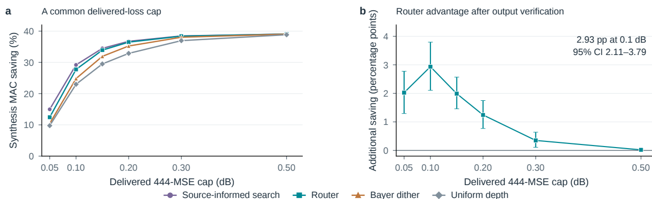
Figure S11. Controlling delivered loss within the recorded candidate pool. a , Maximum saving among actually measured eligible outputs, including a full-frame e15 fallback. b , Paired router–dither difference with 95% sequence-cluster intervals. All 265 pairs are retained, including explicit fallbacks, with YCbCr 4:4:4-loss tolerance 10^{-4} dB. This retrospective source-aware comparison excludes the cost of candidate generation and makes no released-reference or latency claim.
