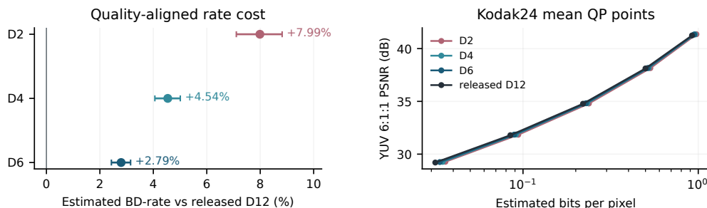
Figure S13. The completed independent codecs approach the release as depth grows. Left, per-image YUV 6:1:1 BD-rate cost on the four-model common PSNR interval; bars are 95% paired-image bootstrap intervals ( n = 24 ). Right, mean five-QP operating points on Kodak24. Rates are deterministic entropy estimates, not actual bitstreams. Released D12 differs in training history from the three scratch models.
