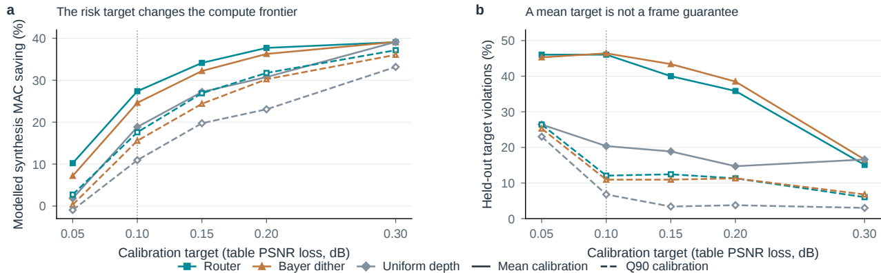
Figure S9. A source-free control trades arithmetic savings against tail risk. Controls are calibrated on other sequences, separately at each QP, using the training mean (solid) or 90th percentile (dashed). All 265 pairs are retained, including cases from infeasible calibration groups. a , Modelled MAC saving. b , Fraction exceeding the table-loss target. These padded source-error diagnostics do not establish final mixed-image quality, a per-frame guarantee or complete decoder speed.
