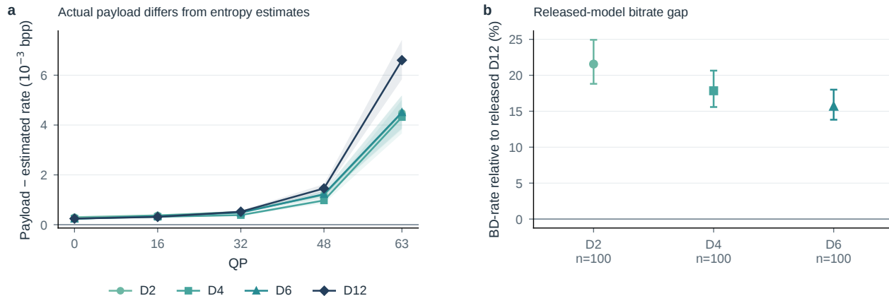
Figure S17. Estimated entropy and emitted bytes are separate quantities. a , Actual rANS payload minus entropy estimate, excluding the research header. b , Mean per-image BD-rate against the released anchor on each image’s four-model common PSNR interval. Intervals resample images; no uncertainty from independent training seeds is represented.
