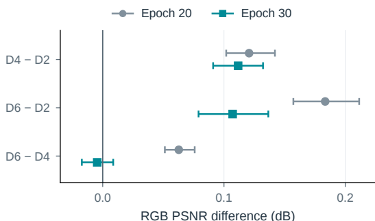
Figure S18. Intermediate depth ordering changes during training. Paired RGB PSNR differences at 0.2 actual payload bpp on the same 99 images. Epochs 20 and 30 are retained without quality-based selection. Intervals are 95% image-bootstrap intervals at fixed weights, excluding training-seed uncertainty. No rate extrapolation.
