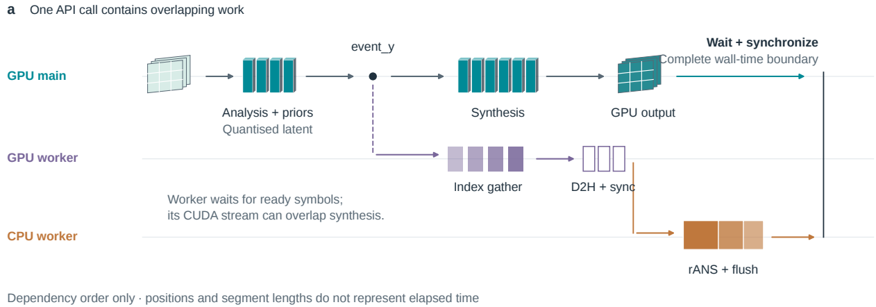
Figure S31. Time the completed workload across streams. Source-derived dependencies of the pinned native DCVC-UF intra encoder. The main-stream reconstruction can overlap worker-stream symbol handling and CPU entropy coding after the latent-ready event. The right boundary includes both the worker wait and completion of the GPU reconstruction. Positions, segment lengths and glyph counts are illustrative, not measured durations or layer counts. This diagram establishes a timing contract, not a speedup.
