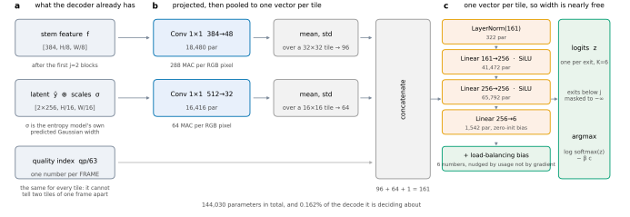
Figure 4. The router head. a, the three things it reads, all already held by the decoder. b, each projected by a 1\times 1 , then reduced to one vector per tile by its mean and standard deviation. c, a three-layer perceptron, one pass per tile. Every shape and parameter count is read off the module when the figure is drawn.
