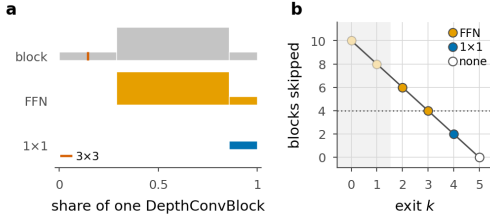
Figure 2. Inside an exit adapter. a, one DepthConvBlock and the two adapters, drawn to scale: bar length is a share of the block, bar height the channel width written. Neither adapter contains the block's only 3\times 3 (the hairline rule), so neither adds receptive field or seam penalty. b, blocks skipped per exit, coloured by adapter; the rule switches to the FFN at four skipped blocks. Lengths counted with hooks off the modules themselves.
