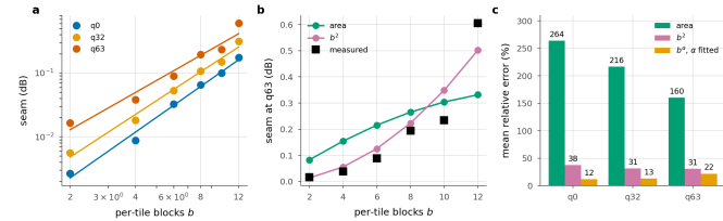
Figure 6. The seam against per-tile depth. a , the measurement with the fitted power law. b , both models against q63, one free scale each. c , mean relative error. The area fraction saturates once the border reaches every pixel; the penalty does not.
