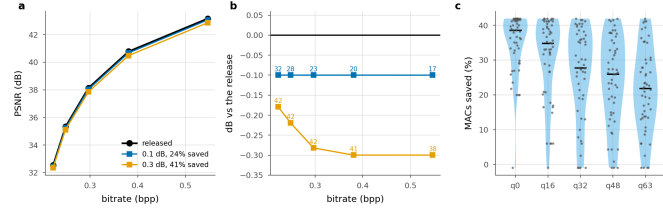
Figure 10. The plane a codec is read on, and the spread behind the mean. a , operating points against the released curve. b , the same with the quality axis expanded; labels are compute saved. c , per sequence at a matched point near 0.1 dB; one dot per sequence, bar is the median.
