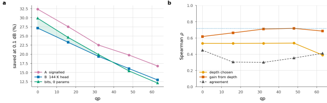
Figure 18. The calibrated bit rule. a Sparing at 0.1 dB; shaded where the calibrated bit rule beats the trained head. b What a tile's bit count is correlated with, against how often the rule agrees with the oracle outright; dotted is the head's own held-out agreement.
