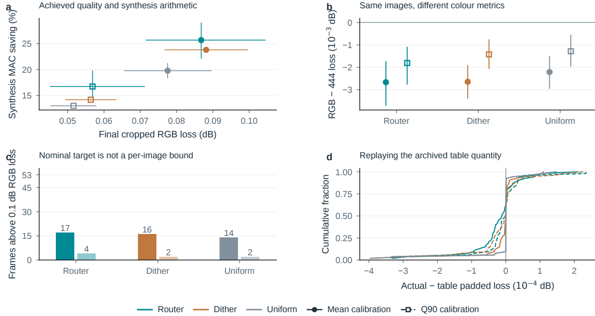
Figure S25. Carry the fixed decision through to the actual image. All 53 sequences at QP32, with no outcome-based exclusions. a , Achieved RGB loss and synthesis MAC saving with conditional 95% sequence-bootstrap intervals; these points are not an equal-quality frontier. b , RGB-minus-444 loss on the same support and reference. c , Counts above the nominal numerical threshold; pale bars denote Q90 calibration. d , Actual-minus-table loss on padded support. Mean and Q90 controls use a different calibration reference and metric from the cropped RGB report. The paired router-dither saving intervals include zero under both controls.
