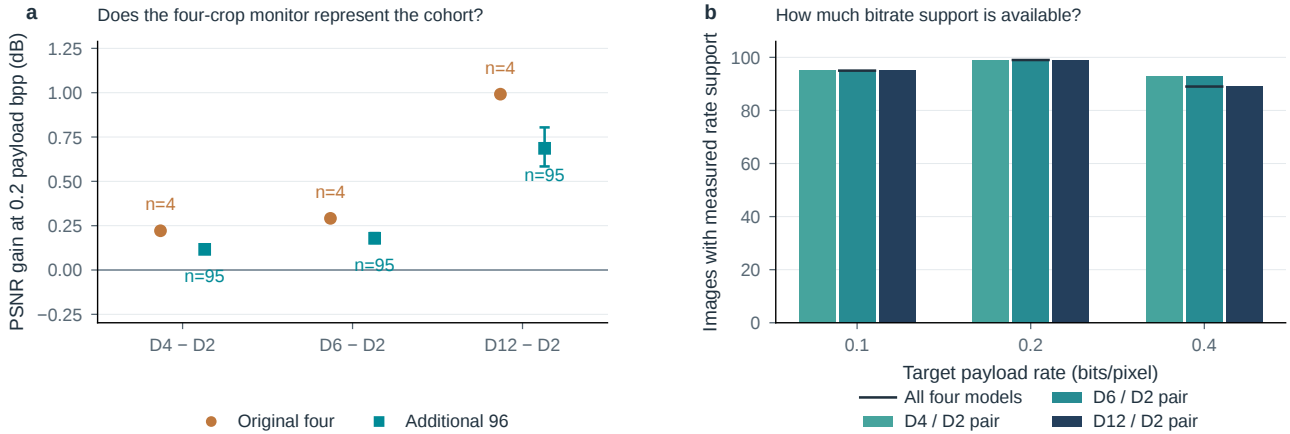
Figure S18. Coverage is part of the result. a , Original monitor crops and additional images at 0.2 payload bpp, restricted to four-model common support. We do not estimate uncertainty from the four-crop subset. b , Pairwise and four-model supported counts at each target rate. A changing cohort is made explicit rather than filled by extrapolation.
