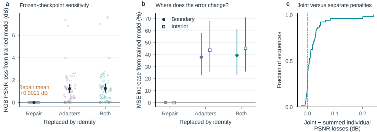
Figure S27. Separate learned dependence from architectural necessity. Fixed QP32, checkpoint and Q90 exit maps on all 53 first frames. a , RGB PSNR loss after identity substitution: individual sequences, means and paired 95% bootstrap intervals. b , Relative MSE change in boundary and interior pixels, averaged within sequence before aggregation. c , Joint-minus-summed individual PSNR penalties. This is a frozen-weight sensitivity test; it measures neither retrained alternatives nor runtime.
