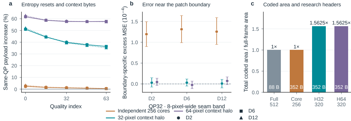
Figure S29. A better seam and a better codec are different outcomes. a , Same-QP payload increase over the full-frame model. b , At QP32, patch-minus-full MSE in the central 8-pixel seam band, minus the corresponding interior excess. c , Exact coded area and research-header bytes. Halo32 and halo64 have equal coded area under this padding policy, but different real context. Area ratios are not latency ratios, and same-QP seam diagnostics are not equal-rate quality comparisons.
