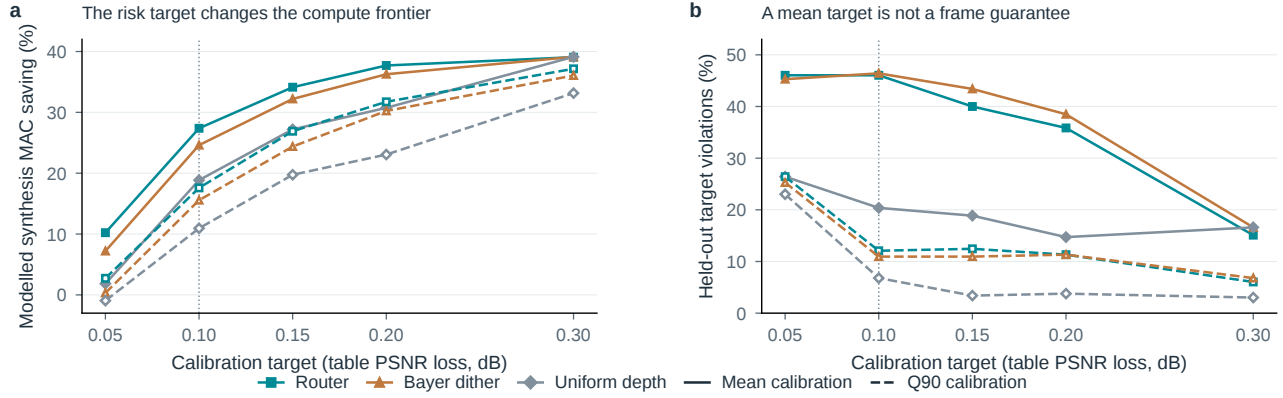
Figure S11. A source-free control trades arithmetic savings against tail risk. Controls are calibrated on other sequences, separately at each QP, using the training mean (solid) or 90th percentile (dashed). All 265 pairs are retained, including cases from infeasible calibration groups. a , Modelled MAC saving. b , Fraction exceeding the table-loss target. These padded source-error diagnostics do not establish final mixed-image quality, a per-frame guarantee or complete decoder speed.
