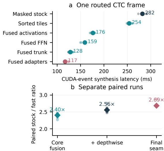
Figure S34. An implementation gain on one real routed frame. a , Six shuffled, paired CUDA-event trials of consecutive kernel stages. Dots are trials and large marks are medians. b , Three separately timed implementations; ratios are paired within each run but cannot be compared as an incremental ablation across runs because GPU contention changed. CTC videoSRC05 at QP32, 1920 \times 1080 valid pixels padded to 2048 \times 1280 , with exit-6/8/10/12 tile counts 13/20/4/3. The GPU was shared with training.
