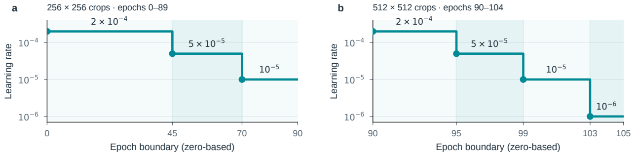
Figure S14. The full official schedule is retained. a , First 90 epochs with 256^2 crops. b , Final 15 epochs with 512^2 crops, on a separately expanded epoch axis. Zero-based boundaries delimit the seven learning-rate stages; the protocol applies to D2/D4/D6. These are prescribed settings, not learning curves.
