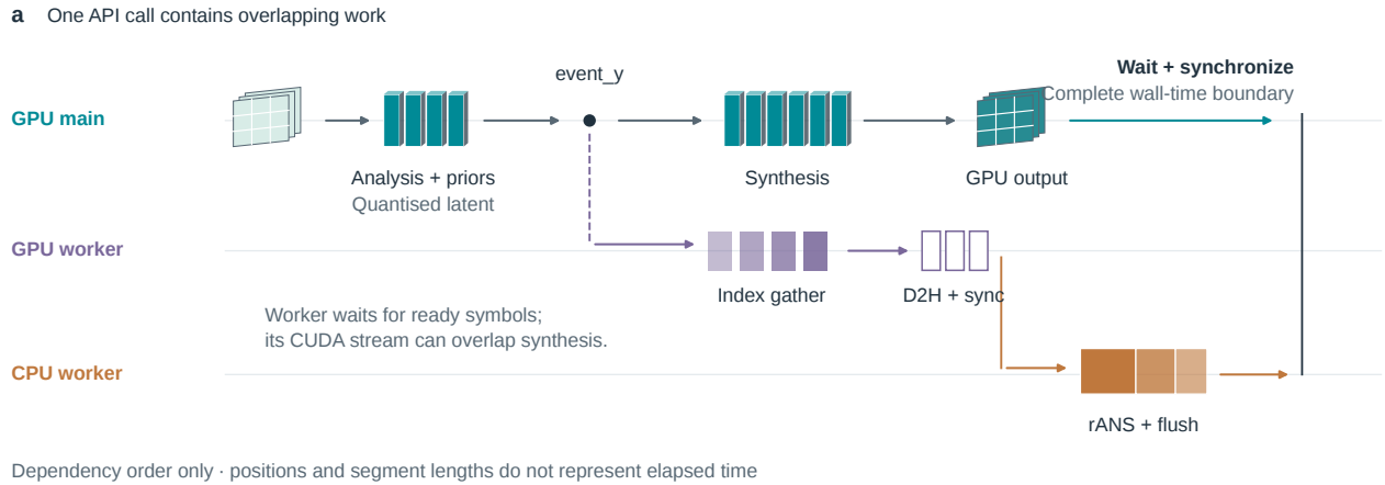
Figure S33. Time the completed workload across streams. Source-derived dependencies of the pinned native DCVC-UF intra encoder. The main-stream reconstruction can overlap worker-stream symbol handling and CPU entropy coding after the latent-ready event. The right boundary includes both the worker wait and completion of the GPU reconstruction. Positions, segment lengths and glyph counts are illustrative, not measured durations or layer counts. This diagram establishes a timing contract, not a speedup.
