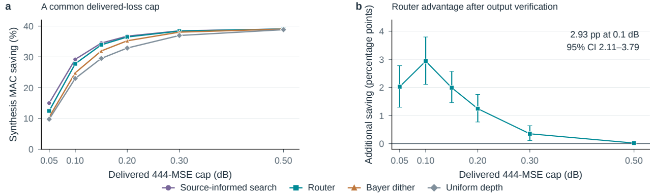
Figure S13. Controlling delivered loss within the recorded candidate pool. a , Maximum saving among actually measured eligible outputs, including a full-frame e15 fallback. b , Paired router–dither difference with 95% sequence-cluster intervals. All 265 pairs are retained, including explicit fallbacks, with YCbCr 4:4:4-loss tolerance 10^{-4} dB. This retrospective source-aware comparison excludes the cost of candidate generation and makes no released-reference or latency claim.
