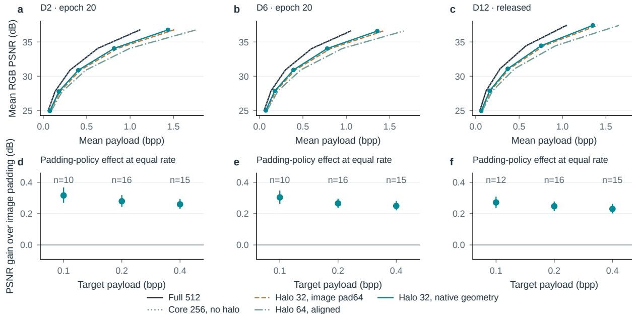
Figure S31. Keep spatial rounding inside the codec contract. a–c, Actual-payload RD points averaged over the fixed 16-image cohort, with shared axis limits. d–f, Per-image matched-rate gain from moving padding to the latent, with paired 95% image-bootstrap intervals. Each rate uses the common support of all five variants within that depth; n denotes supported images out of 16, with no extrapolation. The latent-padding implementation uses CPU FP32 research streams; “native geometry” does not denote native CUDA output or latency.
