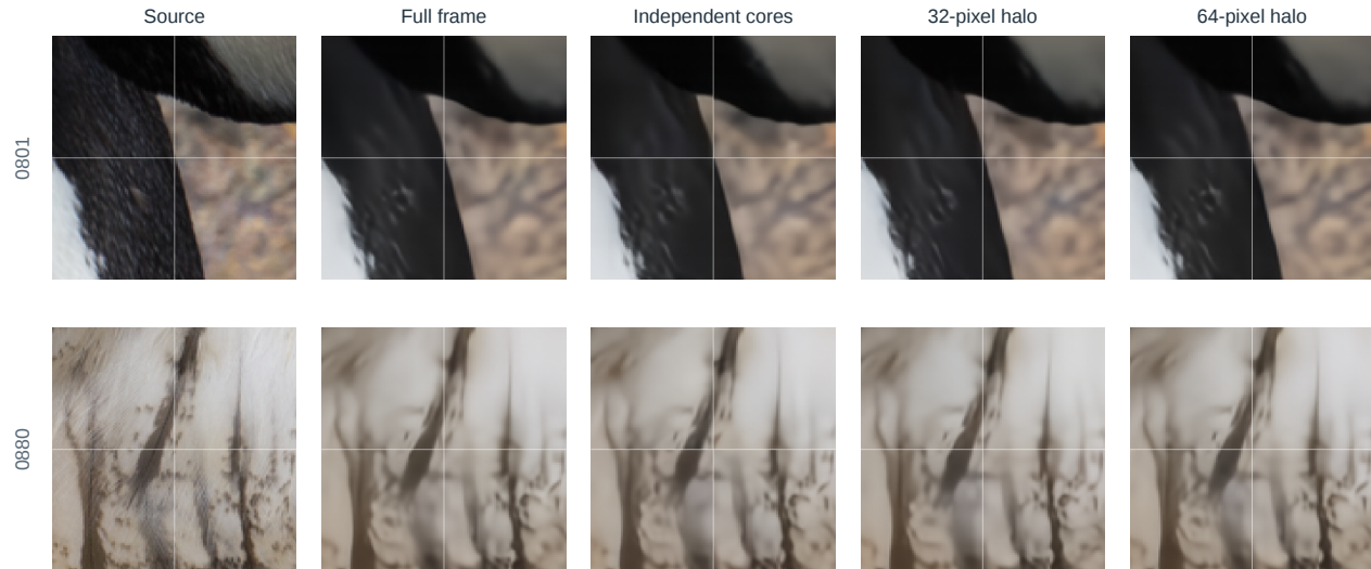
Figure S30. Predeclared views at the region intersection. D6 epoch 20, QP32, DIV2K 0801 and 0880. All panels use rows and columns 192:320 of the same 512-square crop; images and window were fixed before outcomes. The common light cross marks the patch boundary. Display images are rounded to 8 bit; numerical metrics use floating-point RGB. These are same-QP views, not equal-bitrate reconstructions.
