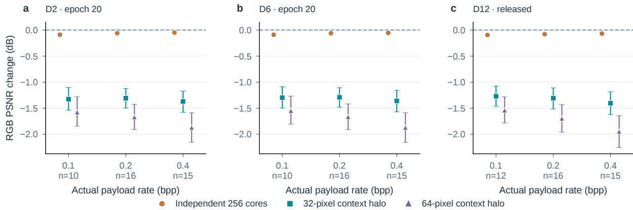
Figure S28. Charge repeated context to the transmitted rate. RGB PSNR changes from the same full-frame model at matched actual payload rate. Each depth uses the common supported images across full frame and all three patch variants; counts are shown and the vertical scale is shared. Intervals resample paired images. D2/D6 are interim epoch 20 models; D12 has different released training provenance. The experiment holds depth fixed within every contrast and makes no adaptive-routing or runtime claim.
