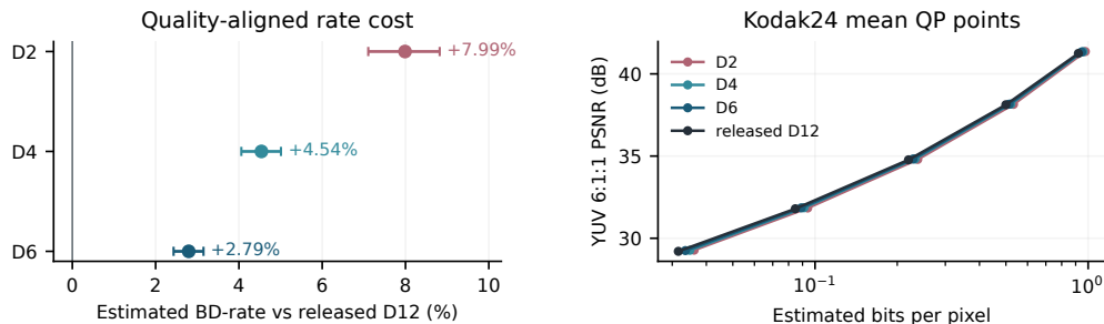
Figure S15. The completed independent codecs approach the release as depth grows. Left, per-image YUV 6:1:1 BD-rate cost on the four-model common PSNR interval; bars are 95% paired-image bootstrap intervals ( n = 24 ). Right, mean five-QP operating points on Kodak24. Rates are deterministic entropy estimates, not actual bitstreams. Released D12 differs in training history from the three scratch models.
