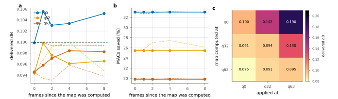
Figure 17. Reusing an exit map. Solid is the transferred map, dashed the one recomputed in place. a , b : reuse across frames of the same sequence. c : reuse across quality index; the entry is the delivered distortion against a 0.1 dB budget.
