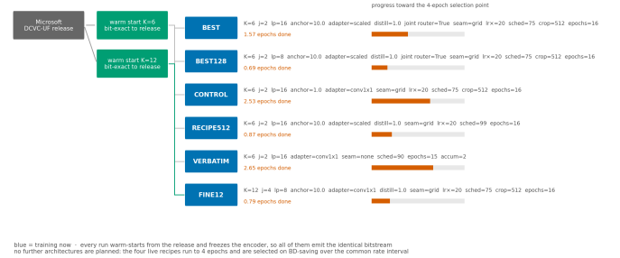
Figure 47. Lineage of the training runs. Every run warm-starts from the released decoder through one of two remaps, one per ladder size, and freezes the encoder, so all of them consume the identical bitstream. The flags shown are the ones that differ between runs. The progress bars are a snapshot taken on 2026-08-18 and the runs have advanced since; the current position of the run this paper reports is given in A.10.
