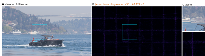
Figure 63. The seam, at frame scale. a the decoded frame. b the absolute error against a full-frame decode of the same latent, amplified 30 \times , with every tile at the deepest exit so that nothing here is early exiting. c a zoom on one junction. The tile grid is the error: 0.124 dB at q63, paid before the allocation begins.
