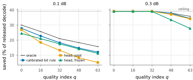
Figure 61. The rule sits between the two heads and the oracle. Saving at each rate, against the Lagrangian oracle measured inside the same run and the architectural ceiling (dotted). At 0.1 dB the rule is above both heads at every rate, and the gap between the two heads is wider than the gap between the rule and either of them. At 0.3 dB the three lowest rates saturate and the three curves separate only at q48 and q63.
