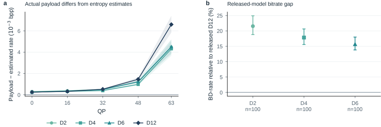
Figure S15. Estimated entropy and emitted bytes are separate quantities. a , Actual rANS payload minus entropy estimate, excluding the research header. b , Mean per-image BD-rate against the released anchor on each image’s four-model common PSNR interval. Intervals resample images; no uncertainty from independent training seeds is represented.
