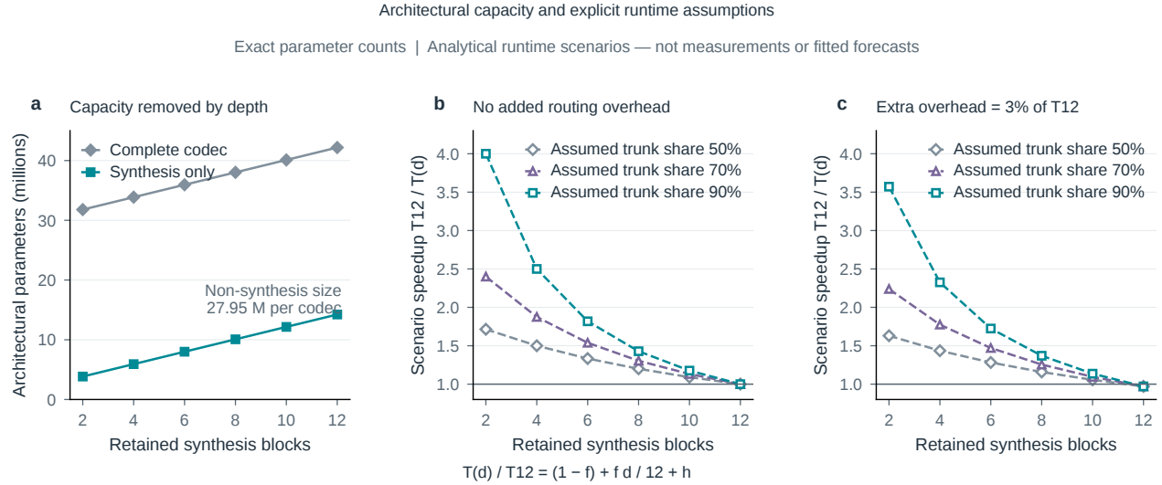
Figure S19. A transparent design-space illustration for unfinished experiments. a , Exact architectural parameter counts. b,c , Analytical runtime sensitivity to assumed trunk-time share and added overhead. Open markers and dashed lines denote assumptions, not measurements or fitted forecasts. No quality or bitrate outcome is assigned to an unfinished model.
