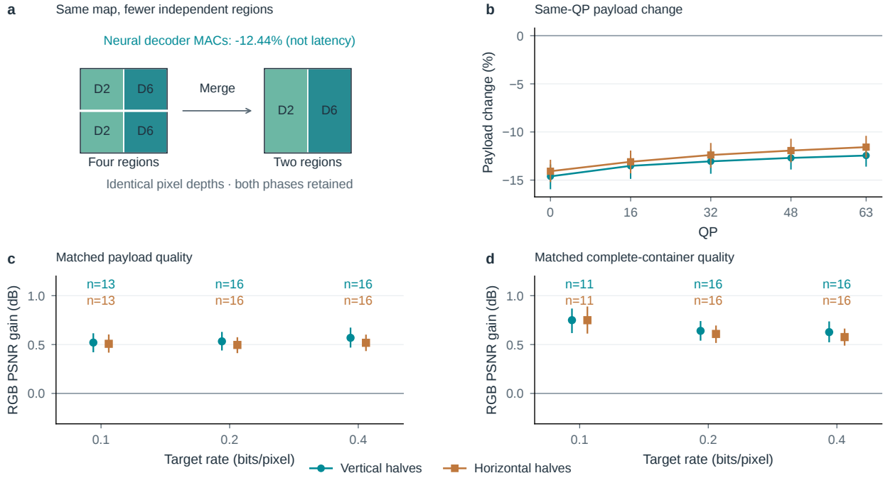
Figure S28. Better region execution without a better selector. a , One phase of the fixed depth-map control; every pixel keeps its D2 or D6 assignment. b , Same-QP relative payload change after coalescing. c,d , RGB PSNR gain at matched payload and complete-container rate, on shared vertical scales. Complementary phases are averaged within image before 95% paired-image bootstrap intervals. Counts show the common support of both phases and implementations, without extrapolation. The 800 outputs include unmerged checkerboards; those have no adjacent same-depth regions to combine. CPU FP32 research streams and epoch-20 weights are used throughout; this is neither learned routing nor a runtime benchmark.
