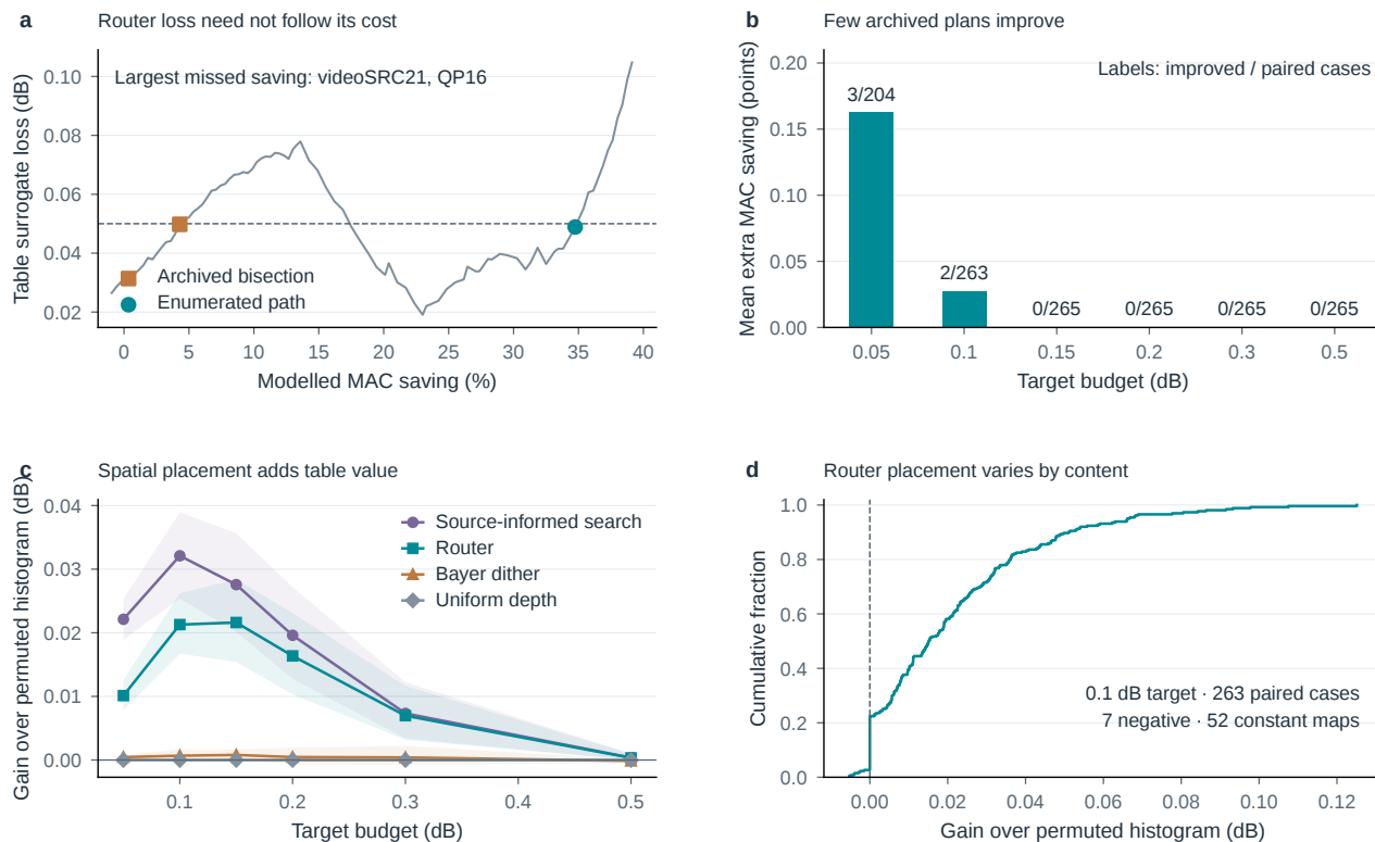
Figure S8. Control-path and assignment diagnostics. a , The explicitly selected largest missed router saving illustrates non-monotone table loss. b , Mean paired improvement from enumerating the router path; labels show improved and paired counts. Newly feasible cases are excluded from these means. c , Exact expected-shuffle comparison at unchanged exit histograms, with 95% sequence-cluster intervals. d , Router placement-gain distribution at 0.1 dB. All results are CPU analyses of padded error tables; none measures new final-image quality or latency.
