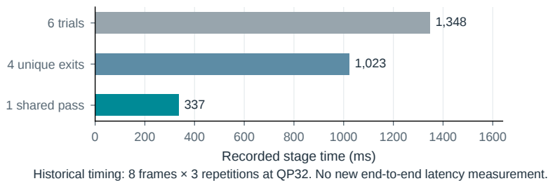
Figure S20. The decision path has an encoder cost. a , Stages required for source-error-based selection, with prefix reuse across candidate exits. b , Historical table-construction upper medians over 24 pooled trials, without invented uncertainty bars. c , A fixed held-out control and per-frame source calibration require different information. This is a stage analysis, not an end-to-end speedup.
