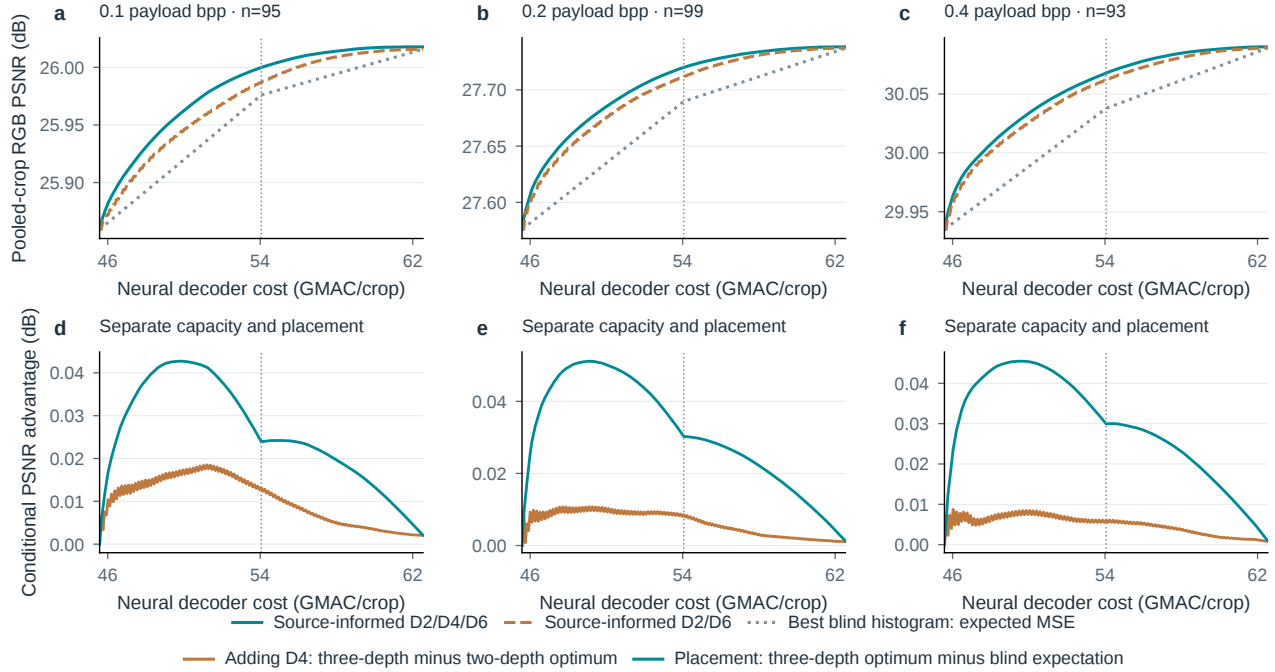
Figure S17. Separate the value of capacity choices from their assignment. Top: exact whole-crop allocation under a shared neural-decoder MAC budget. Bottom: incremental D4 option value and assignment premium over the best source-calibrated blind histogram’s expected MSE. Vertical guides mark the uniform-D4 budget. The curves use interpolated equal-rate quality and contain neither patch entropy resets nor a trained MLP. They are not within-image routing results or runtime frontiers.
