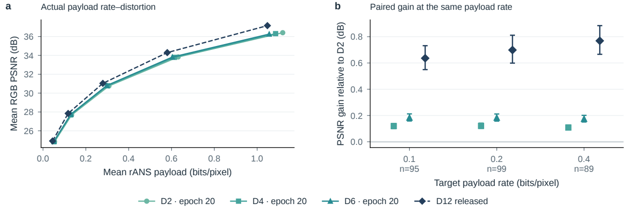
Figure S13. Shallow models are close, but not identical, at equal coded rate. a , Mean RGB PSNR and actual payload over all 100 crops at five QPs; joining lines are visual guides. b , Per-image interpolation and paired differences on four-model common support, with 95% image-bootstrap intervals. D2/D4/D6 are frozen epoch-20 models; released D12 is not matched in training history. These measured streams establish an interim CPU rate–distortion comparison, not final quality or native runtime.
