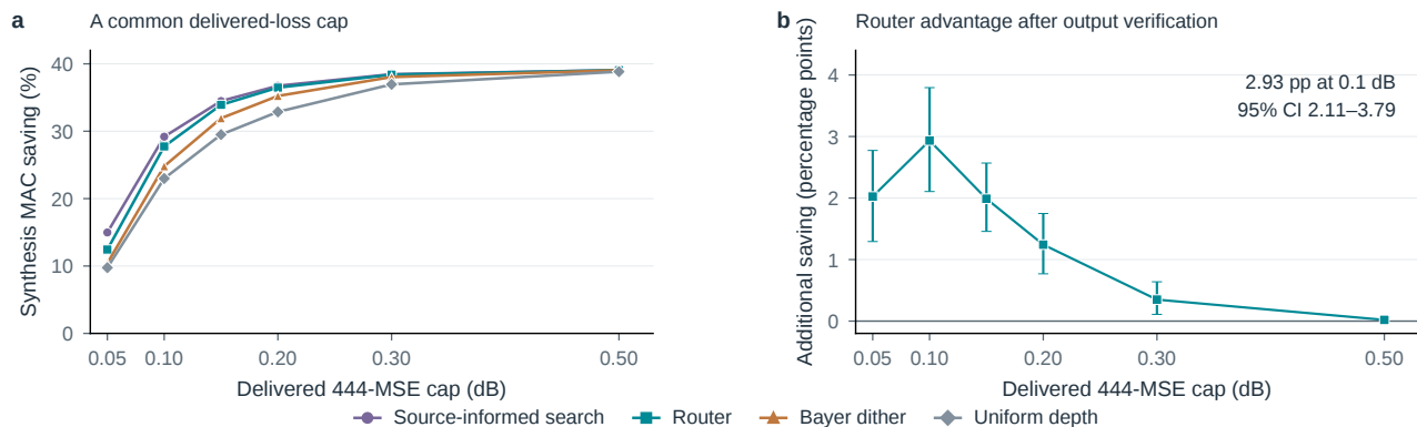
Figure S9. Controlling delivered loss within the recorded candidate pool. a , Maximum saving among actually measured eligible outputs, including a full-frame e15 fallback. b , Paired router–dither difference with 95% sequence-cluster intervals. All 265 pairs are retained, including explicit fallbacks, with YCbCr 4:4:4-loss tolerance 10^{-4} dB. This retrospective source-aware comparison excludes the cost of candidate generation and makes no released-reference or latency claim.
