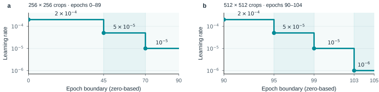
Figure S10. The full official schedule is retained. a , First 90 epochs with 256^2 crops. b , Final 15 epochs with 512^2 crops, on a separately expanded epoch axis. Zero-based boundaries delimit the seven learning-rate stages; the protocol applies to D2/D4/D6. These are prescribed settings, not learning curves.
