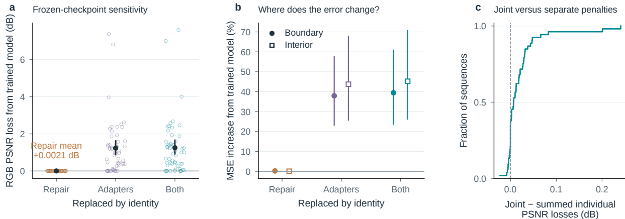
Figure S23. Separate learned dependence from architectural necessity. Fixed QP32, checkpoint and Q90 exit maps on all 53 first frames. a , RGB PSNR loss after identity substitution: individual sequences, means and paired 95% bootstrap intervals. b , Relative MSE change in boundary and interior pixels, averaged within sequence before aggregation. c , Joint-minus-summed individual PSNR penalties. This is a frozen-weight sensitivity test; it measures neither retrained alternatives nor runtime.
