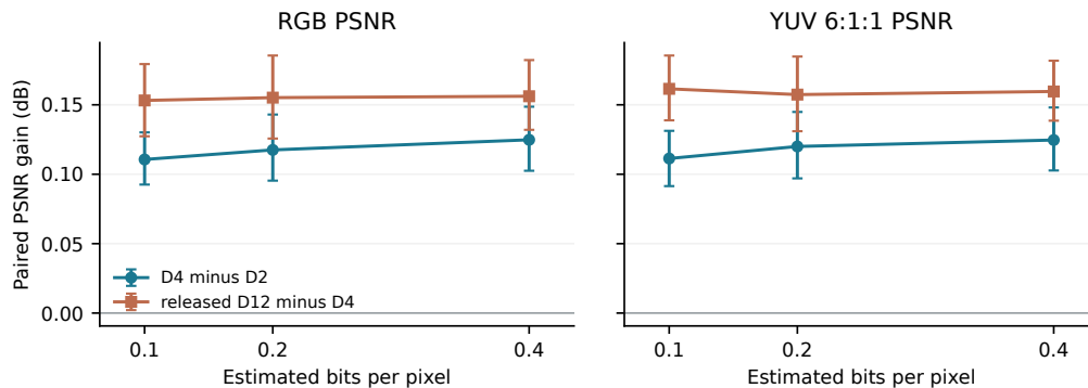
Figure S11. Completed D2/D4 codec quality at matched estimated rate. Image-paired PSNR differences on Kodak after the full 105-epoch official recipe, alongside the released D12 anchor. Rates are interpolated per image in log estimated bpp on common support. Bars show 95% paired-image bootstrap intervals ( n = 24 at 0.1/0.2 bpp; n = 23 at 0.4 bpp). YUV uses the upstream 6:1:1 metric. No actual-bitstream or same-recipe D12 result is implied.
