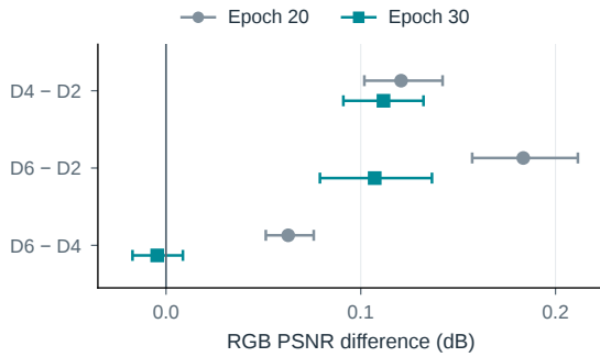
Figure S16. Intermediate depth ordering changes during training. Paired RGB PSNR differences at 0.2 actual payload bpp on the same 99 images. Epochs 20 and 30 are retained without quality-based selection. Intervals are 95% image-bootstrap intervals at fixed weights, excluding training-seed uncertainty. No rate extrapolation.
