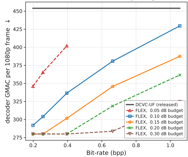
Kodak (decoder complexity)
