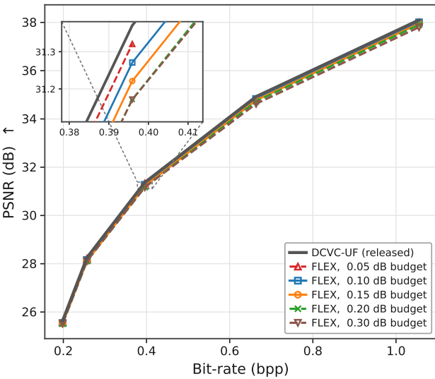
Kodak (PSNR)
