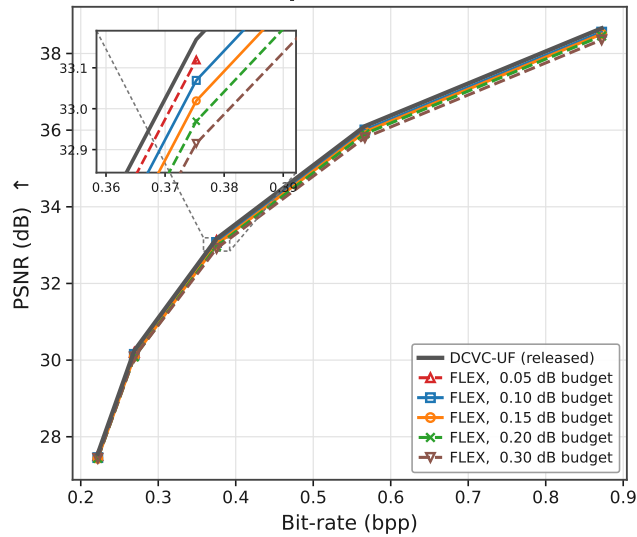
CLIC 2020 professional (PSNR)
