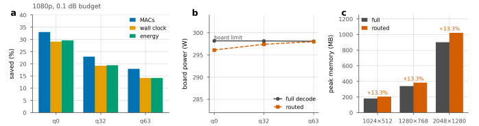
Figure 33. Three units for one saving. a , the same routed decode measured as arithmetic, as wall clock and as joules per frame, at 1080p and a 0.1 dB budget. Energy follows the clock, not the arithmetic. b , why: the board draws the same power either way, because the later groups run on a shrinking set of tiles and a partly idle GPU still draws its static power. c , peak memory, which routing raises rather than lowers, by 13.3% at every resolution that fitted on the card.
