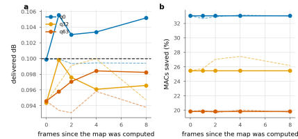
Figure 31. Reusing an exit map. Solid is the transferred map, dashed the one recomputed in place. a , b : reuse across frames of the same sequence. c : reuse across quality index; the entry is the delivered distortion against a 0.1 dB budget.
