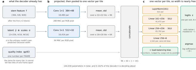
Figure 9. The router head. a , the three things it reads, all already held by the decoder. b , each projected by a 1×1, then reduced to one vector per tile by its mean and standard deviation. c , a three-layer perceptron, one pass per tile. Every shape and parameter count is read off the module when the figure is drawn.
