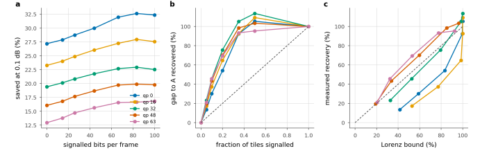
Figure 29. Partial signalling. a , saving against the bits spent on the map; each line runs from B on the left to A on the right. b , the same normalised by the A-to-B gap; dashed is proportional recovery. c , against the fixed- \lambda Lorenz bound; points above the dashed line are allocations one multiplier cannot reach.
