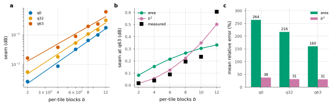
Figure 4. The seam against per-tile depth. Sweeping the split depth sweeps b ; b=0 is an exact control and measures 0.0000 dB at all three rates. a , the measurement with the fitted power law. b , both models against q_{63} with one free scale each. c , mean relative error. The area fraction saturates once every pixel is contaminated; the penalty does not.
