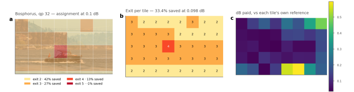
Figure 6. Where the decoder spends. (a) the assignment overlaid on the frame, (b) the exit index per tile, (c) the quality each tile gives up against its own full-depth reference. Water and sky leave at the shallowest rung; the boat and shoreline run deep.
